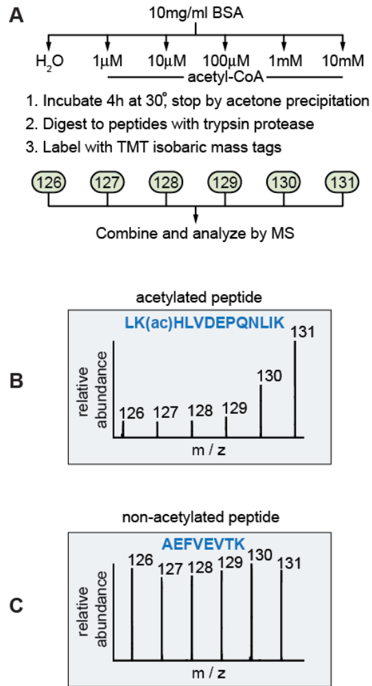
Figure S3. Nonenzymatic acetylation by acetyl-CoA. (A) Diagram showing the experimental conditions and quantitative method using TMT isobaric mass tags. (B) Plot showing a representative MS/MS scan of the indicated acetylated peptide. The region containing the TMT reporter ions is shown. (C) Plot showing a representative MS/MS scan and TMT reporter ions for an unmodified peptide as in panel B.
