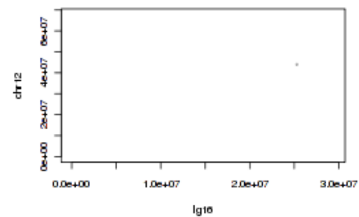
Tobacco Ig16 and tomato chr12
