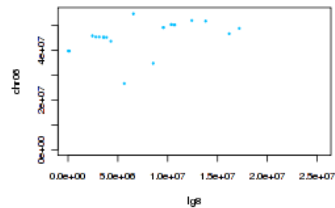
Tobacco Ig8 and tomato chr06
