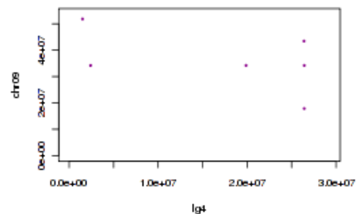
Tobacco lg4 and tomato chr09
