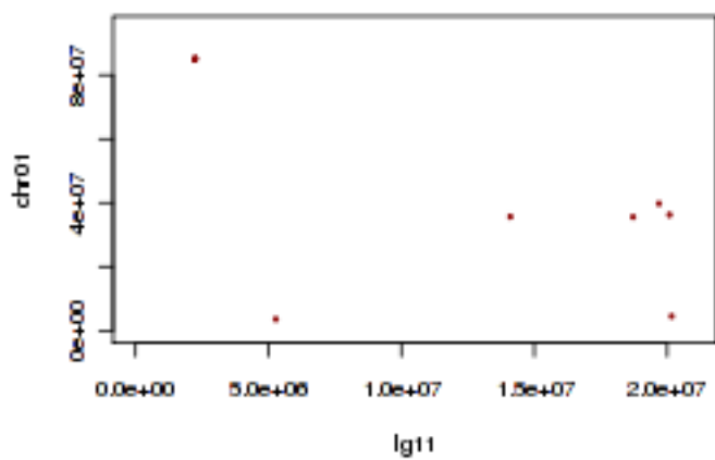
Tobacco lg11 and tomato chr01
