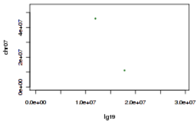
Tobacco lg19 and tomato chr07
