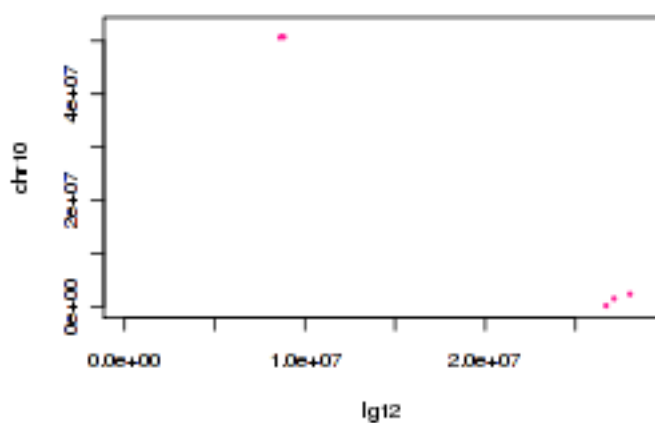
Tobacco lg12 and tomato chr10
