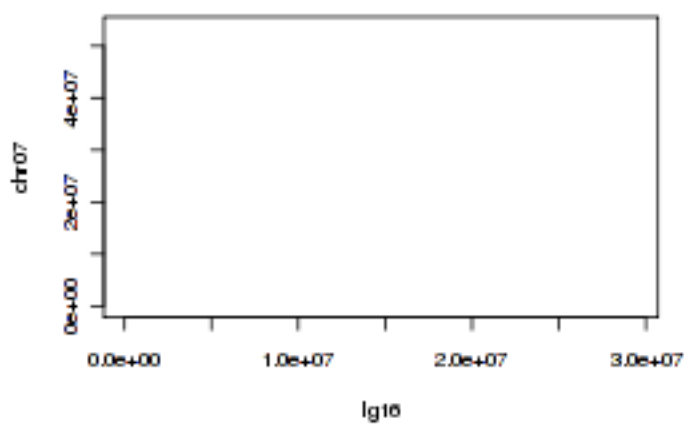
Tobacco Ig16 and tomato chr07
