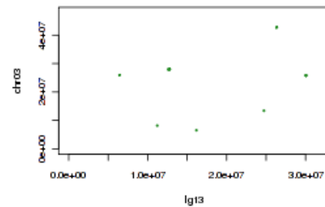
Tobacco lg13 and tomato chr03
