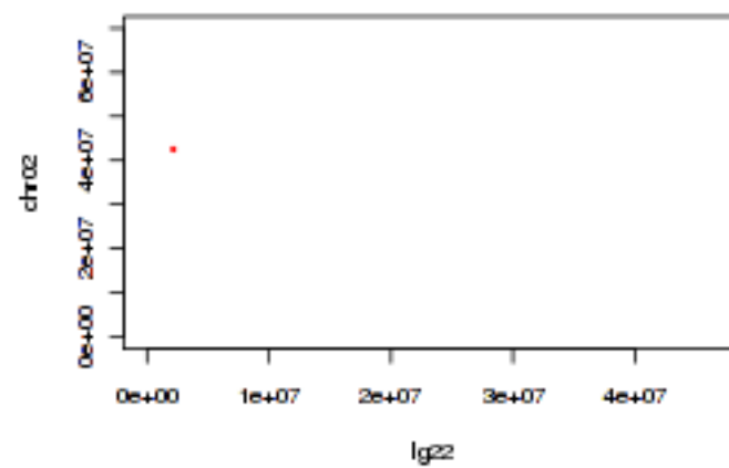
Tobacco Ig22 and tomato chr02
