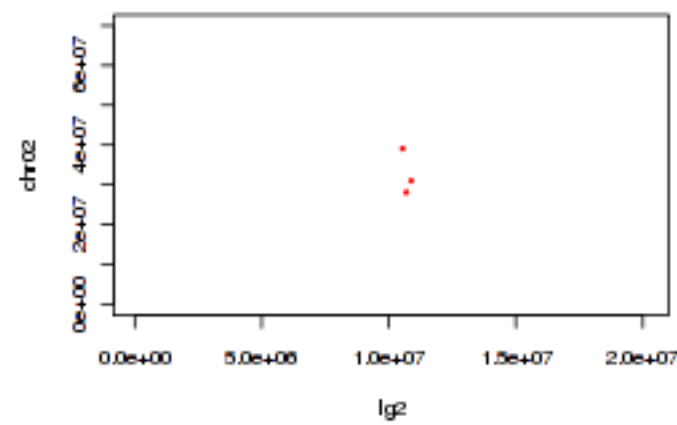
Tobacco lg2 and tomato chr02
