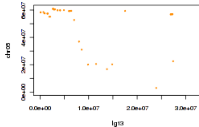
Tobacco lg13 and tomato chr05
