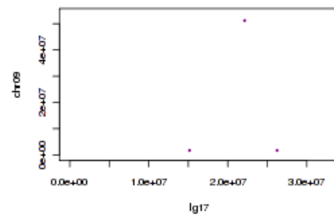
Tobacco lg17 and tomato chr09
