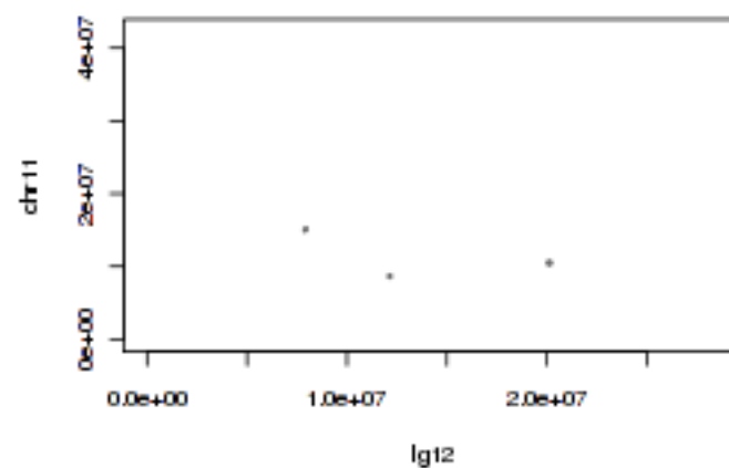
Tobacco lg12 and tomato chr11
