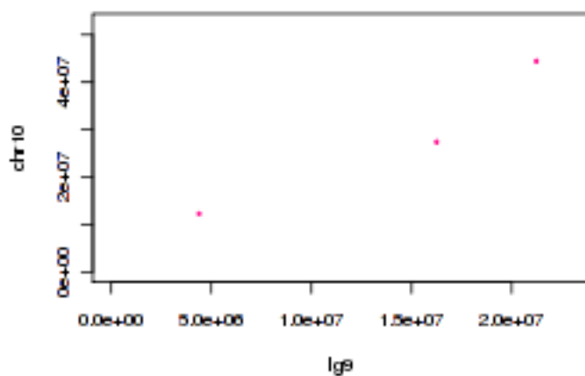
Tobacco Ig9 and tomato chr10
