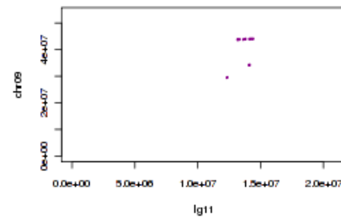
Tobacco lg11 and tomato chr09
