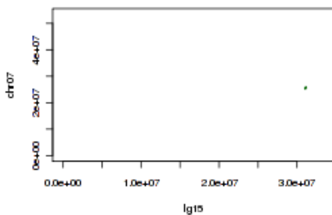
Tobacco lg15 and tomato chr07
