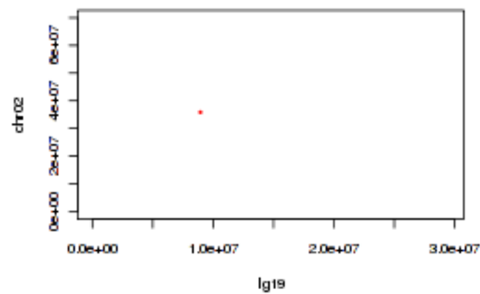
Tobacco lg19 and tomato chr02
