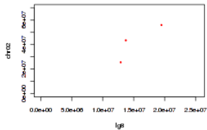
Tobacco Ig8 and tomato chr02
