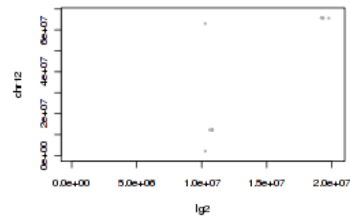
Tobacco lg2 and tomato chr12
