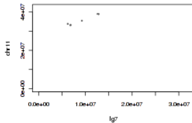
Tobacco lg7 and tomato chr11
