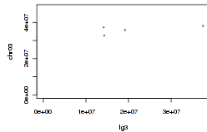
Tobacco Ig3 and tomato chr03
