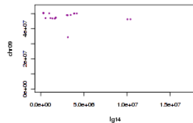
Tobacco lg14 and tomato chr09
