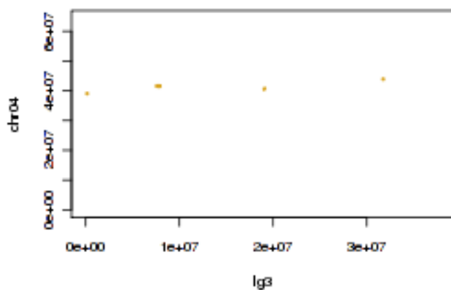
Tobacco Ig3 and tomato chr04
