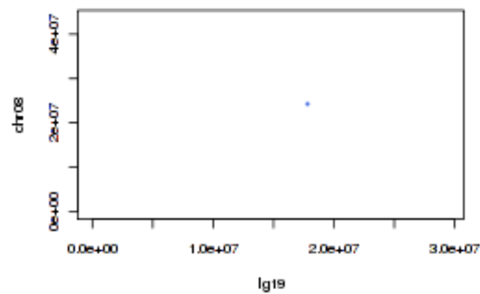
Tobacco lg19 and tomato chr08
