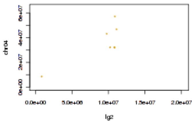
Tobacco lg2 and tomato chr04
