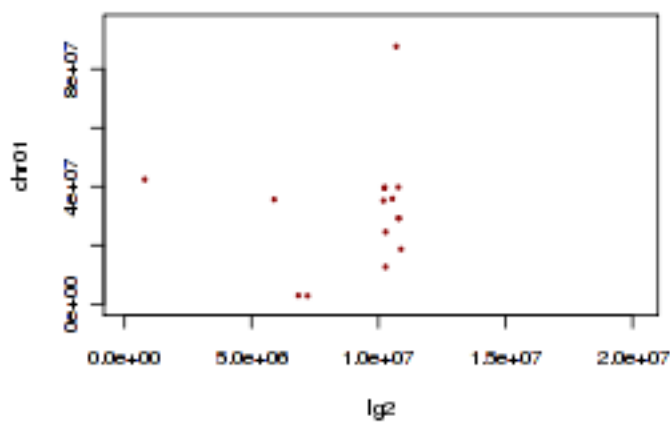
Tobacco lg2 and tomato chr01
