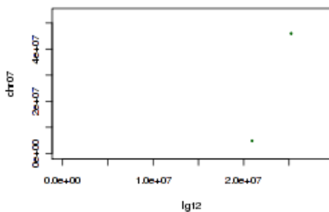
Tobacco lg12 and tomato chr07
