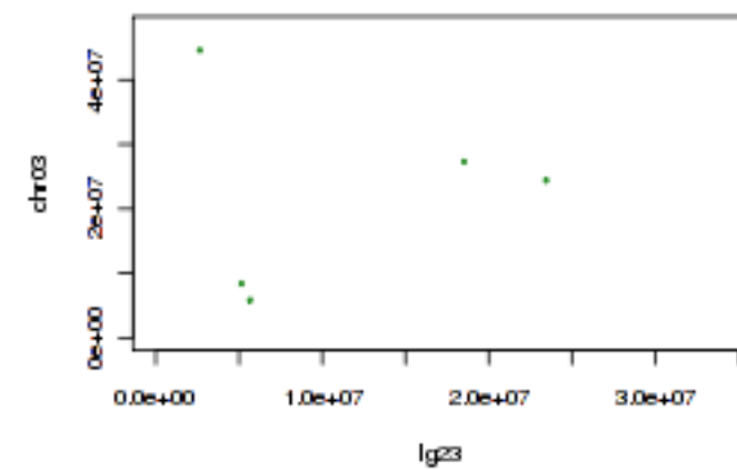
Tobacco Ig23 and tomato chr03
