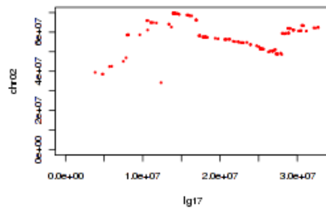
Tobacco lg17 and tomato chr02
