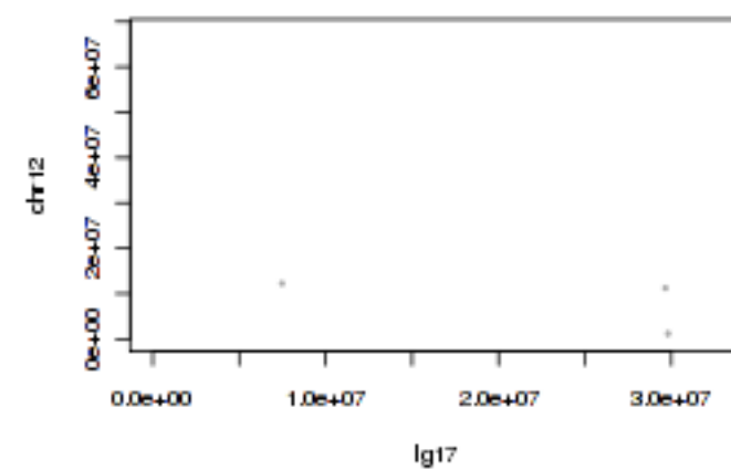
Tobacco lg17 and tomato chr12
