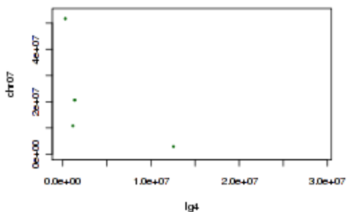
Tobacco lg4 and tomato chr07
