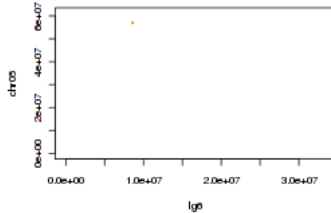
Tobacco IgG and tomato chr05
