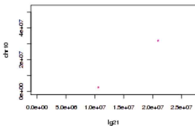
Tobacco lg21 and tomato chr10
