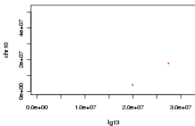
Tobacco lg13 and tomato chr10
