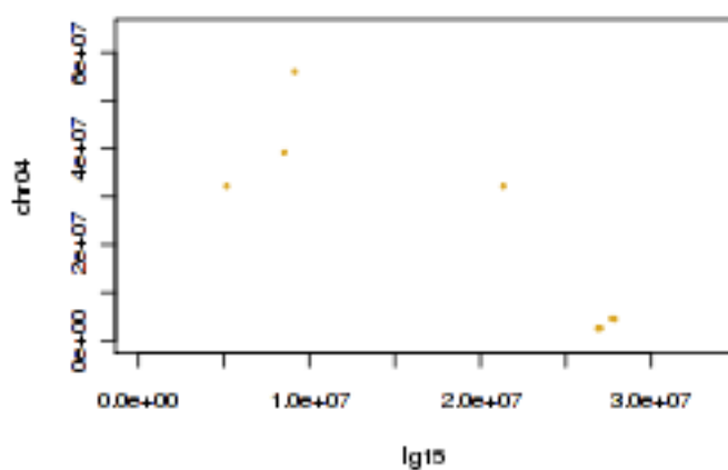
Tobacco lg15 and tomato chr04
