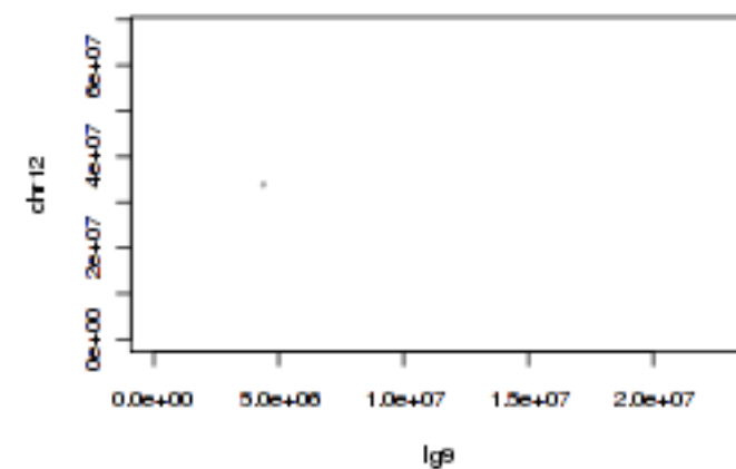
Tobacco Ig9 and tomato chr12
