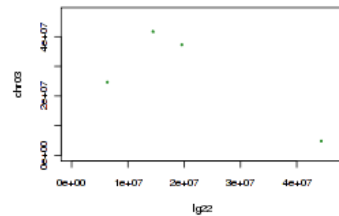
Tobacco Ig22 and tomato chr03
