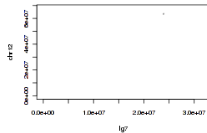
Tobacco lg7 and tomato chr12
