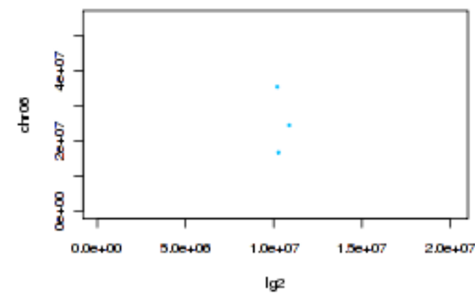
Tobacco lg2 and tomato chr06
