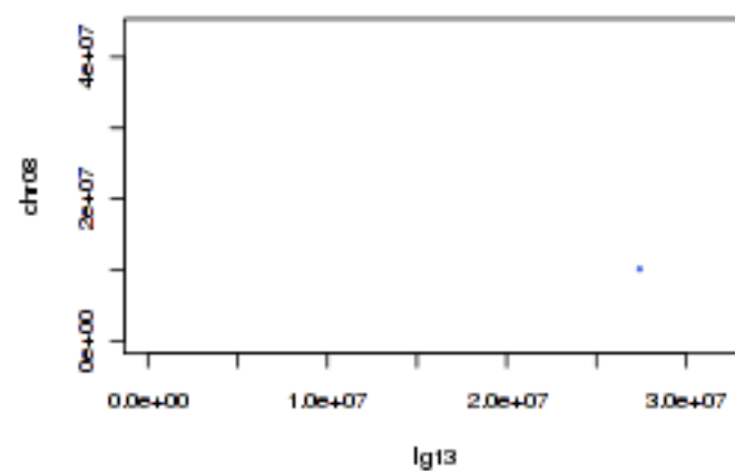
Tobacco lg13 and tomato chr08
