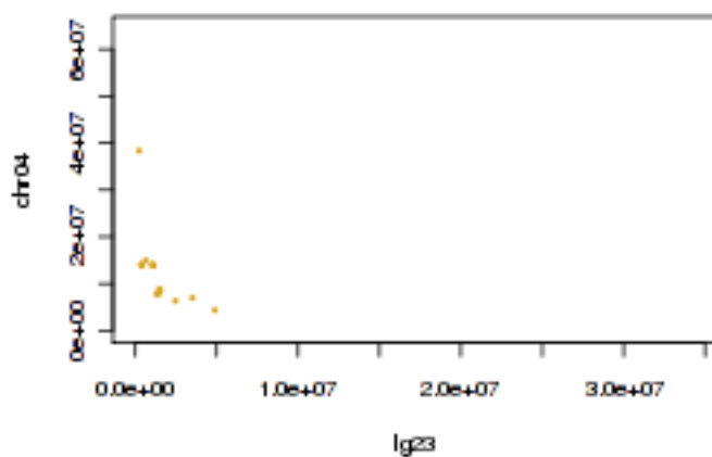
Tobacco Ig23 and tomato chr04
