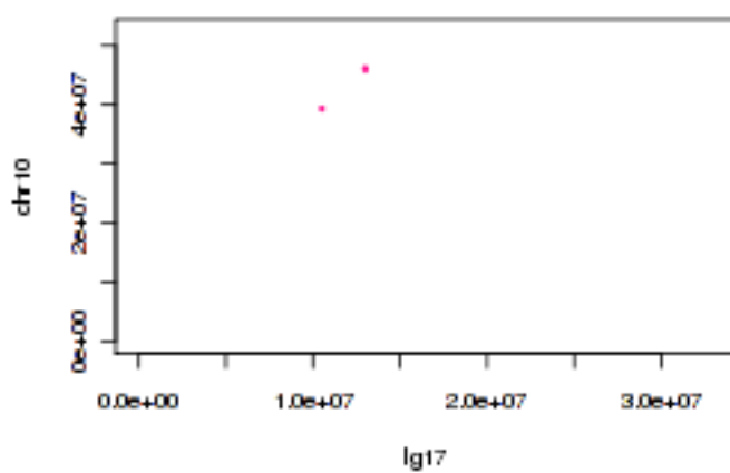
Tobacco lg17 and tomato chr10
