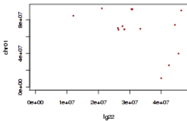
Tobacco Ig22 and tomato chr01
