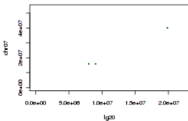
Tobacco Ig20 and tomato chr07
