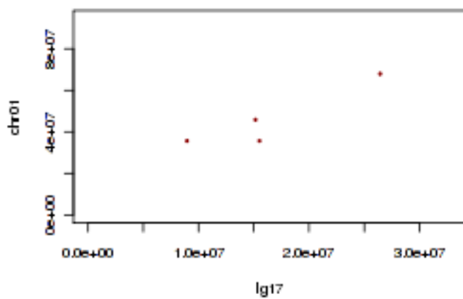
Tobacco lg17 and tomato chr01
