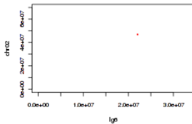
Tobacco IgG and tomato chr02
