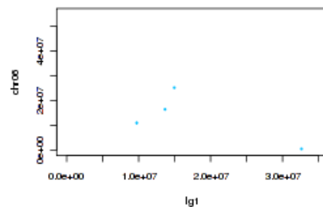
Tobacco lg1 and tomato chr06
