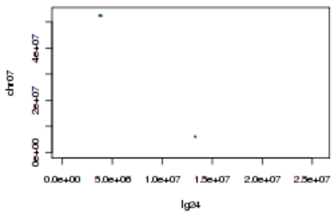
Tobacco Ig24 and tomato chr07
