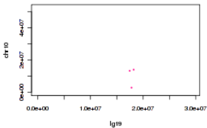
Tobacco lg19 and tomato chr10
