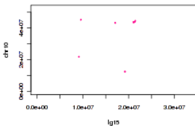
Tobacco lg15 and tomato chr10
