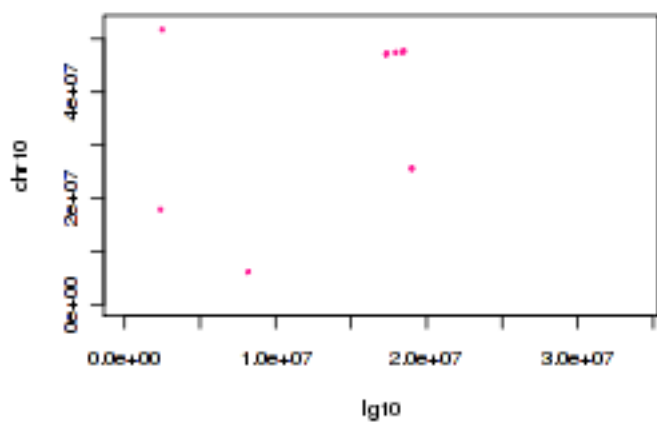
Tobacco lg10 and tomato chr10
