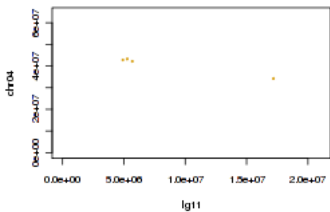
Tobacco lg11 and tomato chr04
