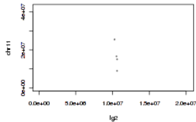
Tobacco lg2 and tomato chr11
