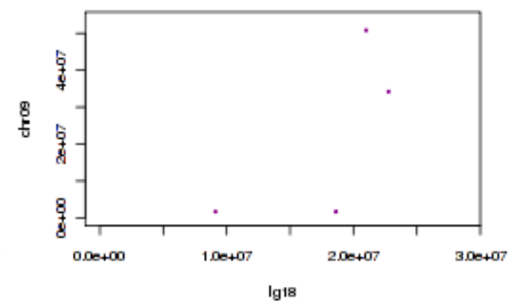
Tobacco lg18 and tomato chr09
