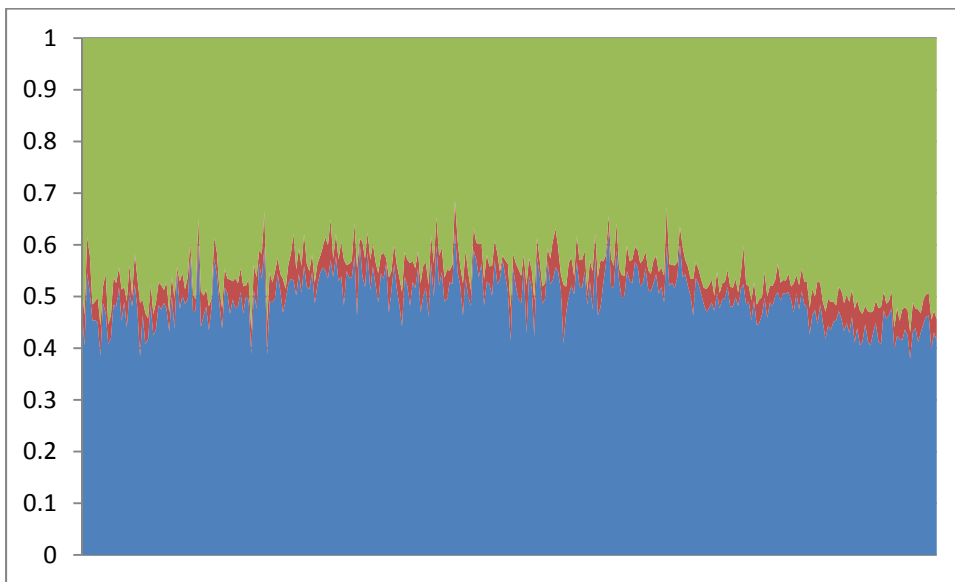
Figure S3 A graphical depiction of RIL Genotype proportions across the 14 chromosomes. Here blue = IM/IM, red = IM/PR (H), and green = PR/PR.
