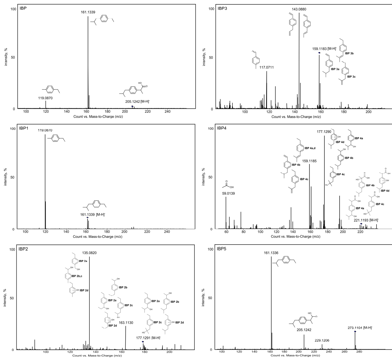
Fig. S1. Mass spectra obtained for ibuprofen and its TPs during the photodegradation experiment
