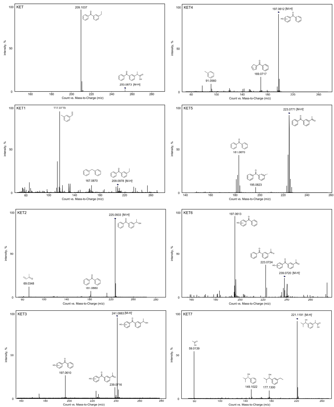
Fig. S2. Mass spectra obtained for ketoprofen and its TPs during the photodegradation experiment
