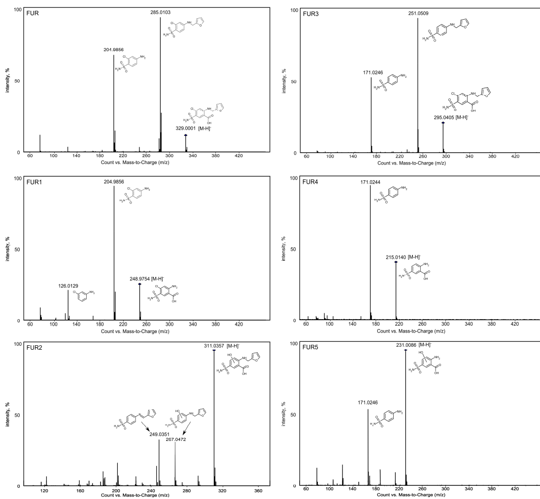
Fig. S3. Mass spectra obtained for furosemide and its TPs during the photodegradation experiment
