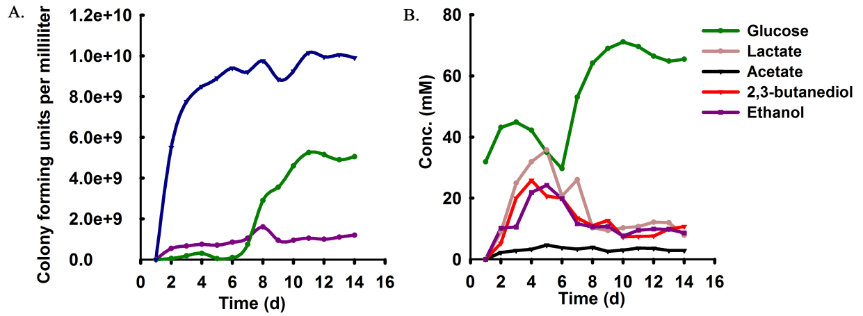
Figure S2. Biological replicate of Figure 2: (A) tracking the population of S. marcescens (purple) in a co-culture with P. aeruginosa (green) over the operating period, and the population of a pure culture of S. marcescens (blue) under similar operating conditions; and (B) metabolite profile of a co-culture of S. marcescens and P. aeruginosa
