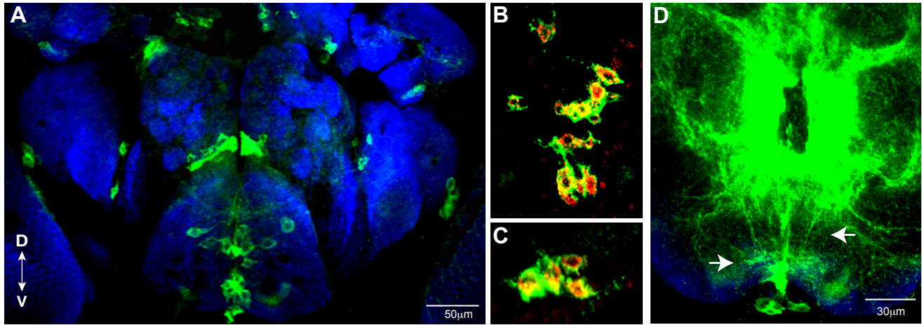
Supplementary Figure S1 (Andrews et al.). Characterization of the Tdc2-LexA line
