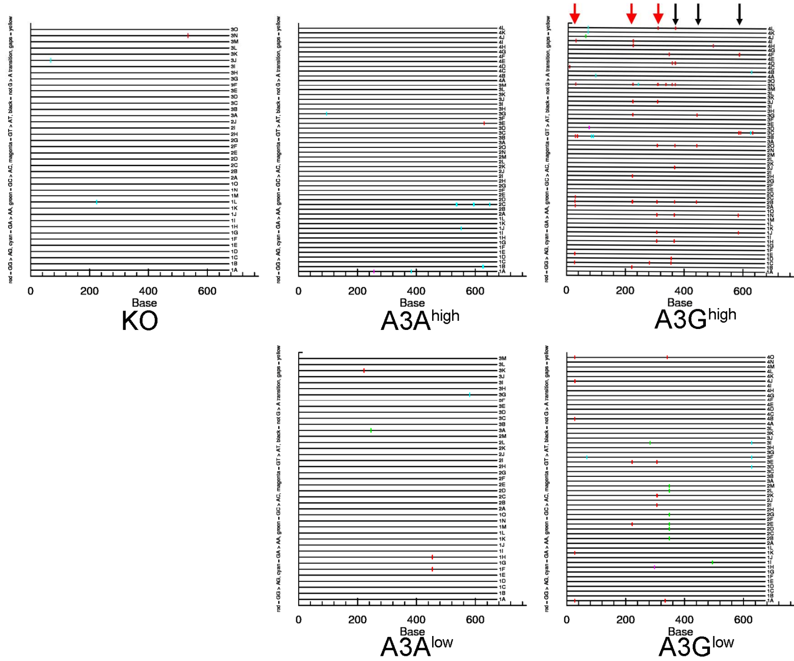
Figure S3. Deamination of MMTV viral DNA in A3A and A3G transgenic mice.
