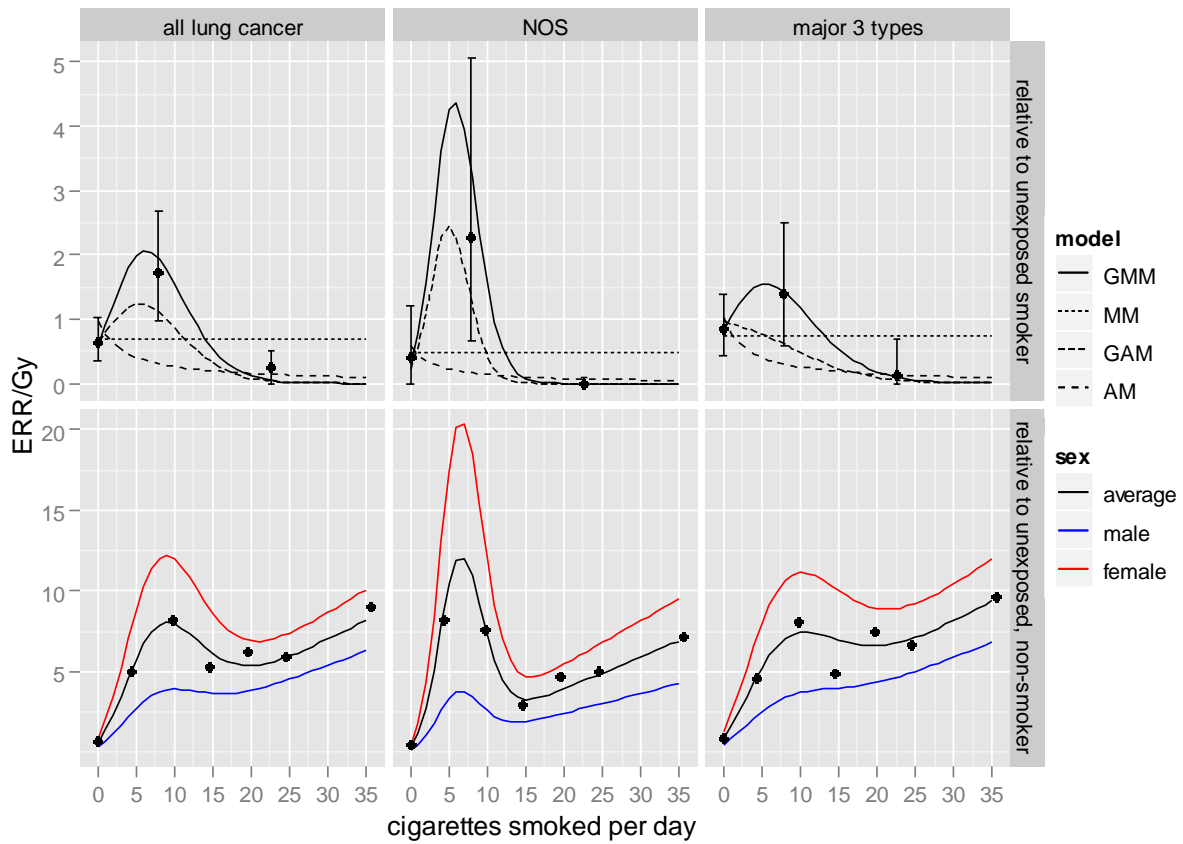
Figure S2. Excess relative risk at 1 Gy as a function of smoking intensity, relative to unexposed smokers with the same smoking history (upper panel) and to unexposed non-smokers (lower panel). The curves correspond to risk at age 70, for one exposed at age 30 who smoked a pack/day for 50 years since age 20. In the upper panel, the gender-averaged risks were plotted for each fitted interaction model. In the lower panel, the gender-averaged and gender-specific risks were plotted for the GMM. All points are based on a GMM in which smoking intensity categories replaced the linear-quadratic function of log intensity.
