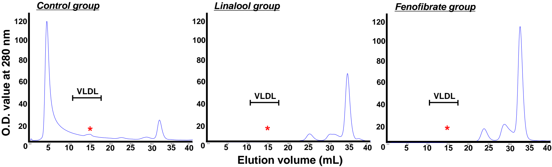
Supplemental Fig. 4. Lipoprotein profiling analysis by FPLC in the plasma of C57BL/6J (A) and apoE2 mice (B). Western diet-fed C57BL/6J and apoE2 mice were orally administered with vehicle, linalool (100 mg/kg body weight/day) or fenofibrate (100 mg/kg body weight/day) for 3 weeks. *VLDL-TG peak.
