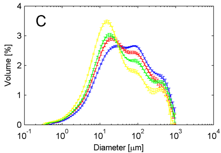
Volume-based particle-size distribution during enzymatic hydrolysis of spruce at 13% WIS. (A) Impeller speed of 100 rpm. (B) Impeller speed of 300 rpm. (C) Impeller speed of 600 rpm. Markers: blue line 0h, red line 4h, green line 24h, yellow line 96h.
