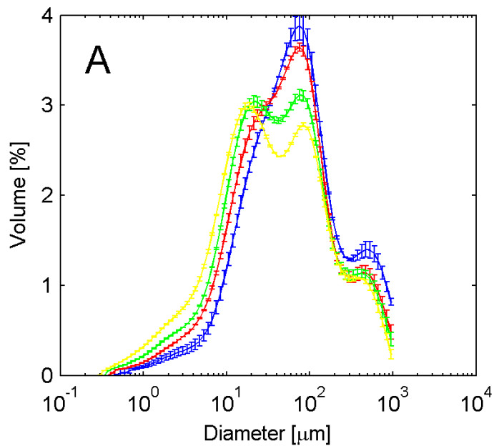
Volume-based particle-size distribution during enzymatic hydrolysis of giant reed at 13% WIS. (A) Impeller speed of 100 rpm. (B) Impeller speed of 300 rpm. Markers: blue line 0h, red line 4h, green line 24h, yellow line 96h.
