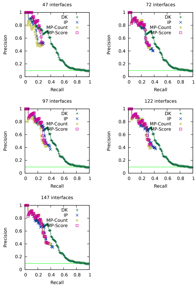
BMV Hit Prediction: Comparison between objective functions (our work: IP) (cycles disallowed, \alpha=0.9 , using literature interactions)
