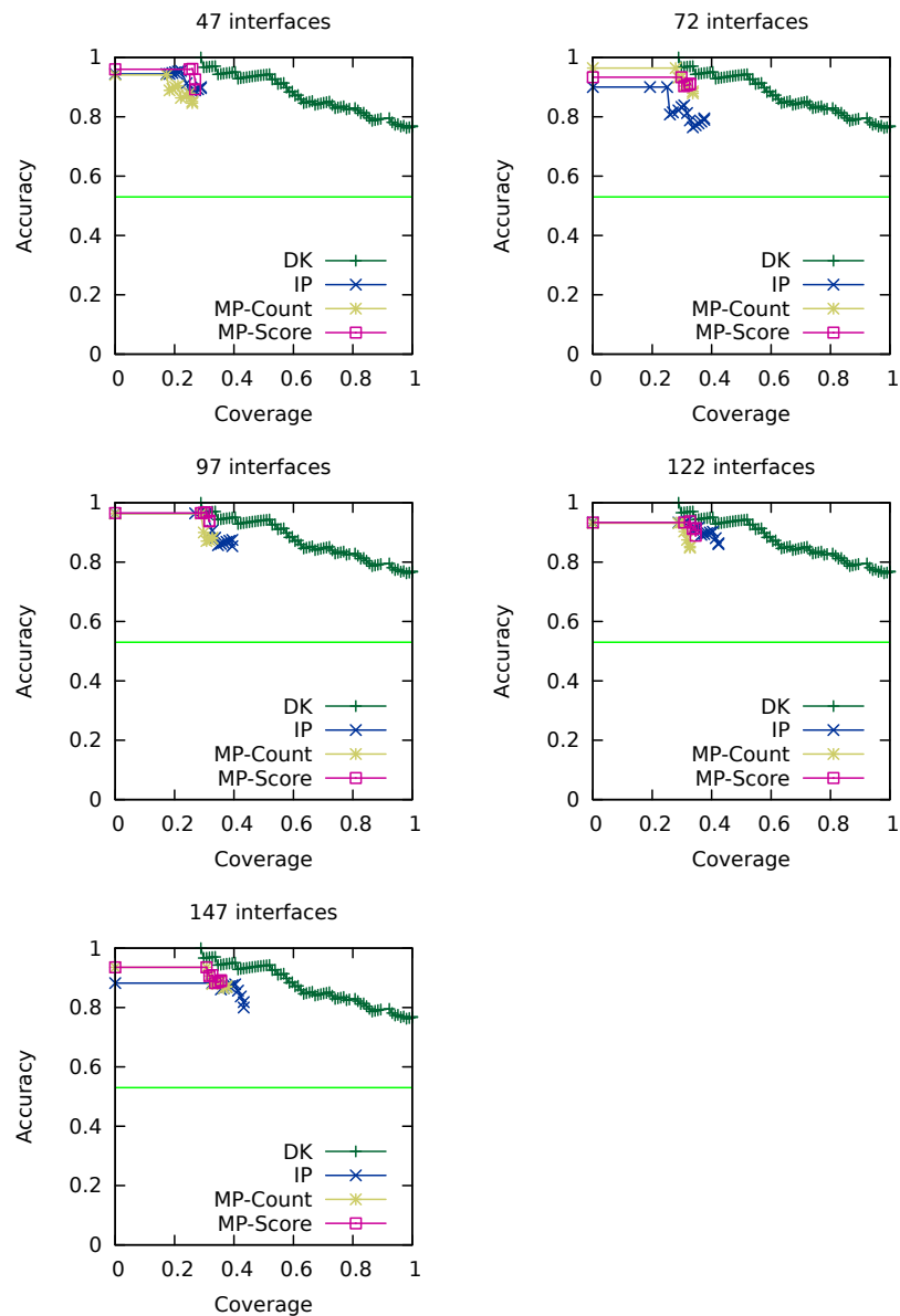
BMV Sign Prediction: Comparison between objective functions (our work: IP) (cycles disallowed, \alpha=0.9 , using literature interactions)
