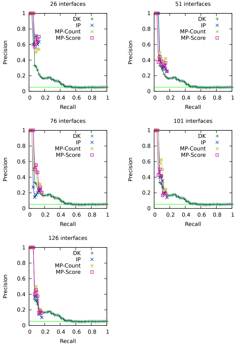
FHV Hit Prediction: Comparison between objective functions (our work: IP) (cycles disallowed, \alpha=0.9 )
