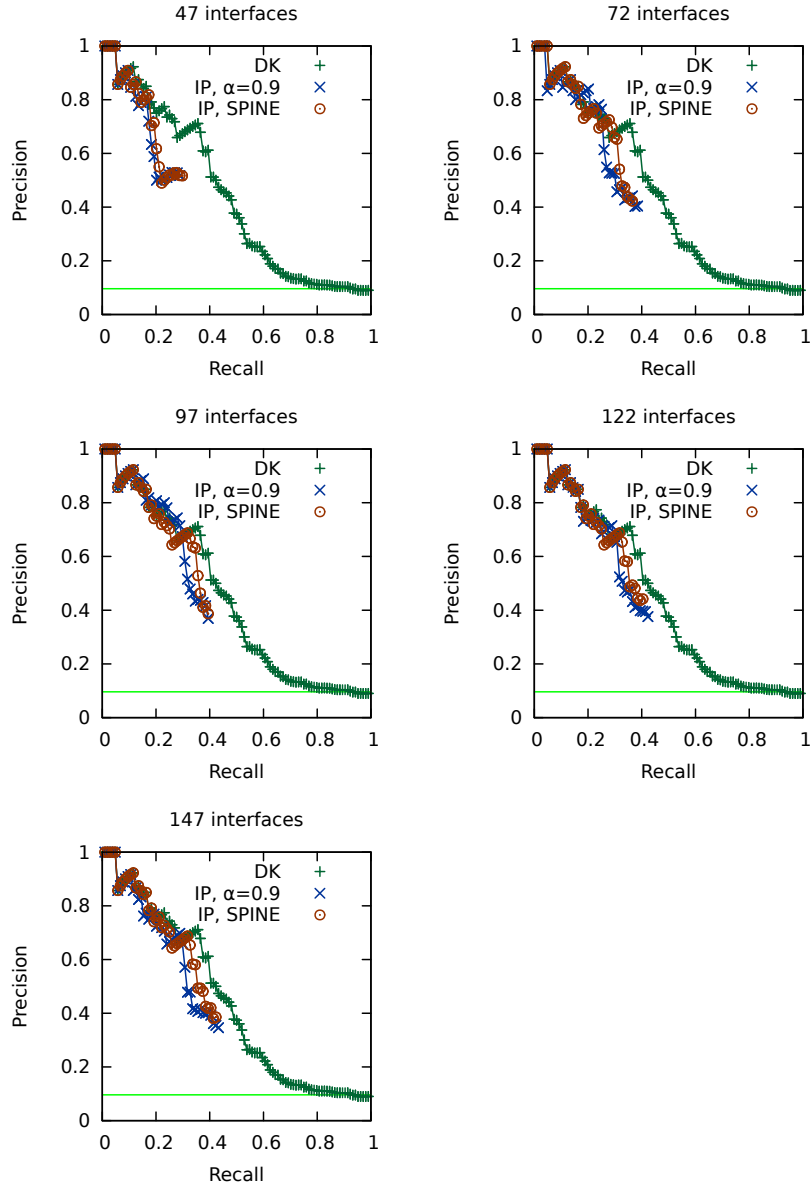
BMV Hit Prediction: IP with \alpha=0.9 (our work) vs. IP with SPINE heuristic (cycles disallowed, using literature interactions)
