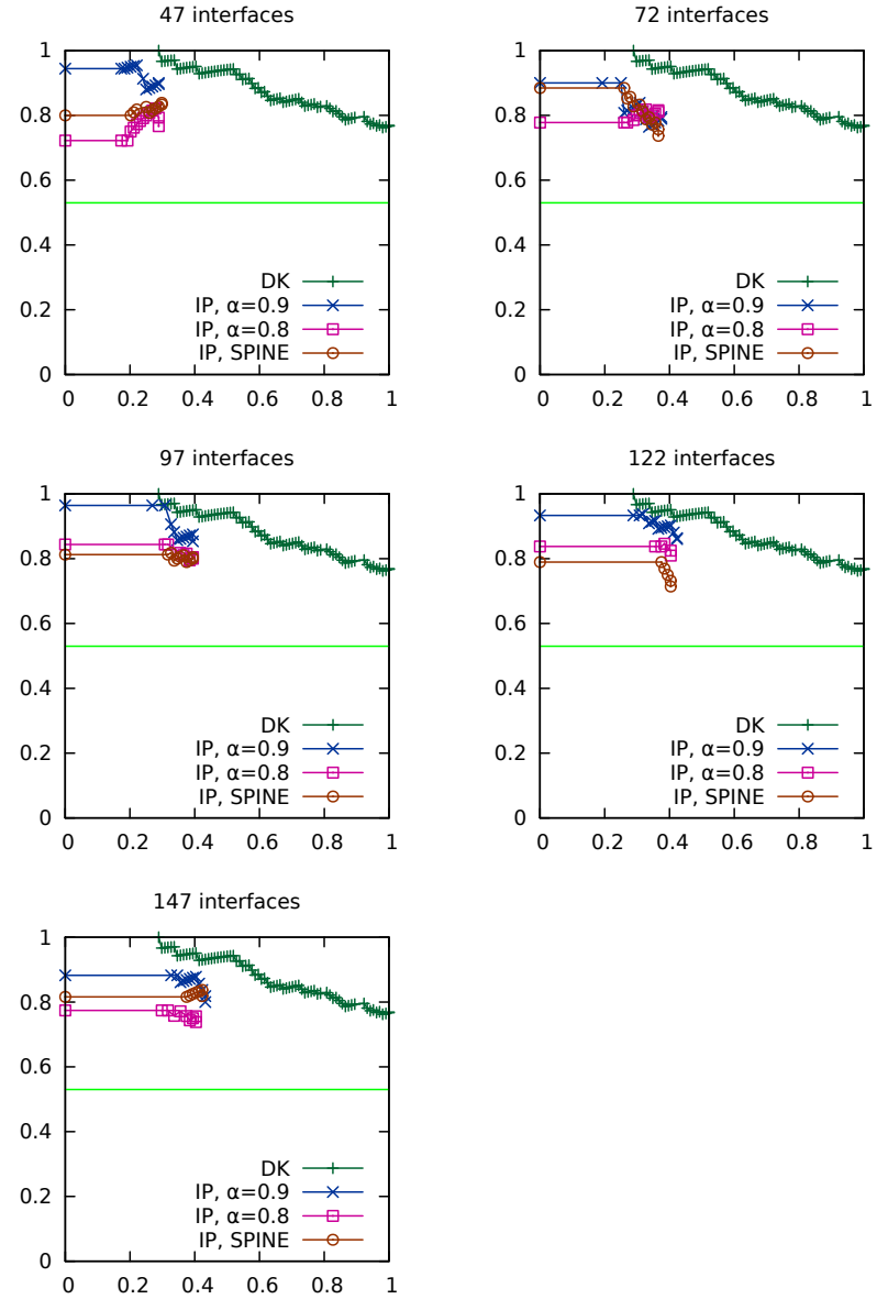
BMV Sign Prediction: IP with \alpha=0.9 (our work) vs. IP with SPINE heuristic (cycles disallowed, using literature interactions)
