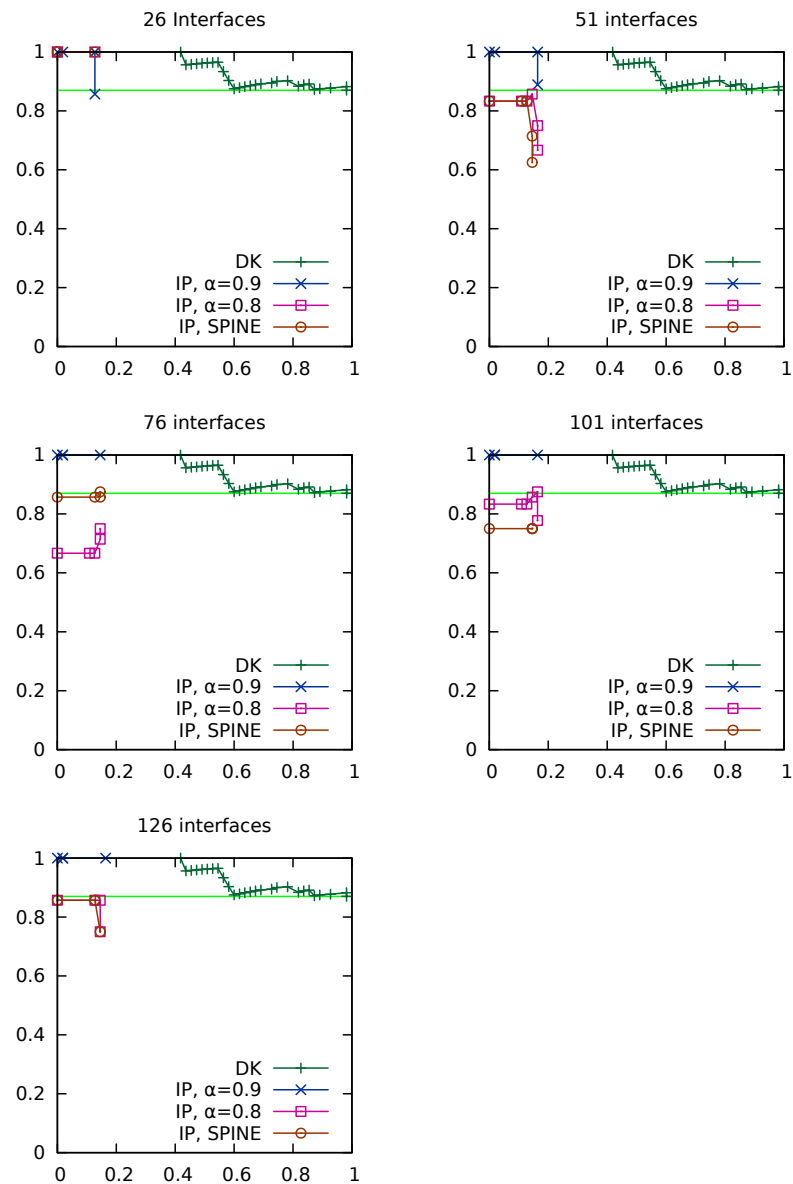
FHV Sign Prediction: IP with \alpha=0.9 (our work) vs. IP with SPINE heuristic (cycles disallowed)
