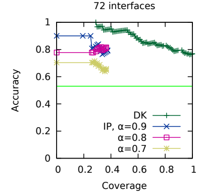
BMV Sign Prediction: Varying \alpha , the proportion of activating edges (using literature interactions, cycles disallowed)
