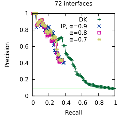
BMV Hit Prediction: Varying \alpha (using literature interactions, cycles disallowed)
