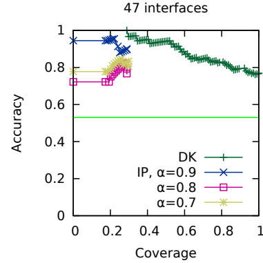
BMV Sign Prediction: Varying \alpha , the proportion of activating edges (using literature interactions, cycles disallowed)
