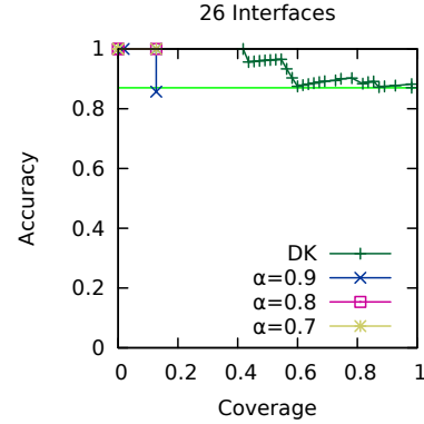
FHV Sign Prediction: Varying \alpha , the proportion of activating edges (cycles disallowed)
