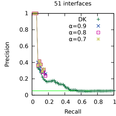
FHV Hit Prediction: Varying \alpha (cycles disallowed)
