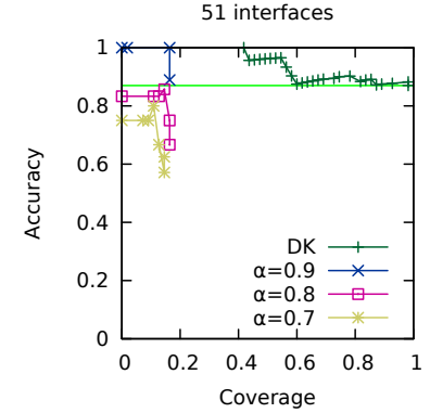
FHV Sign Prediction: Varying \alpha , the proportion of activating edges (cycles disallowed)
