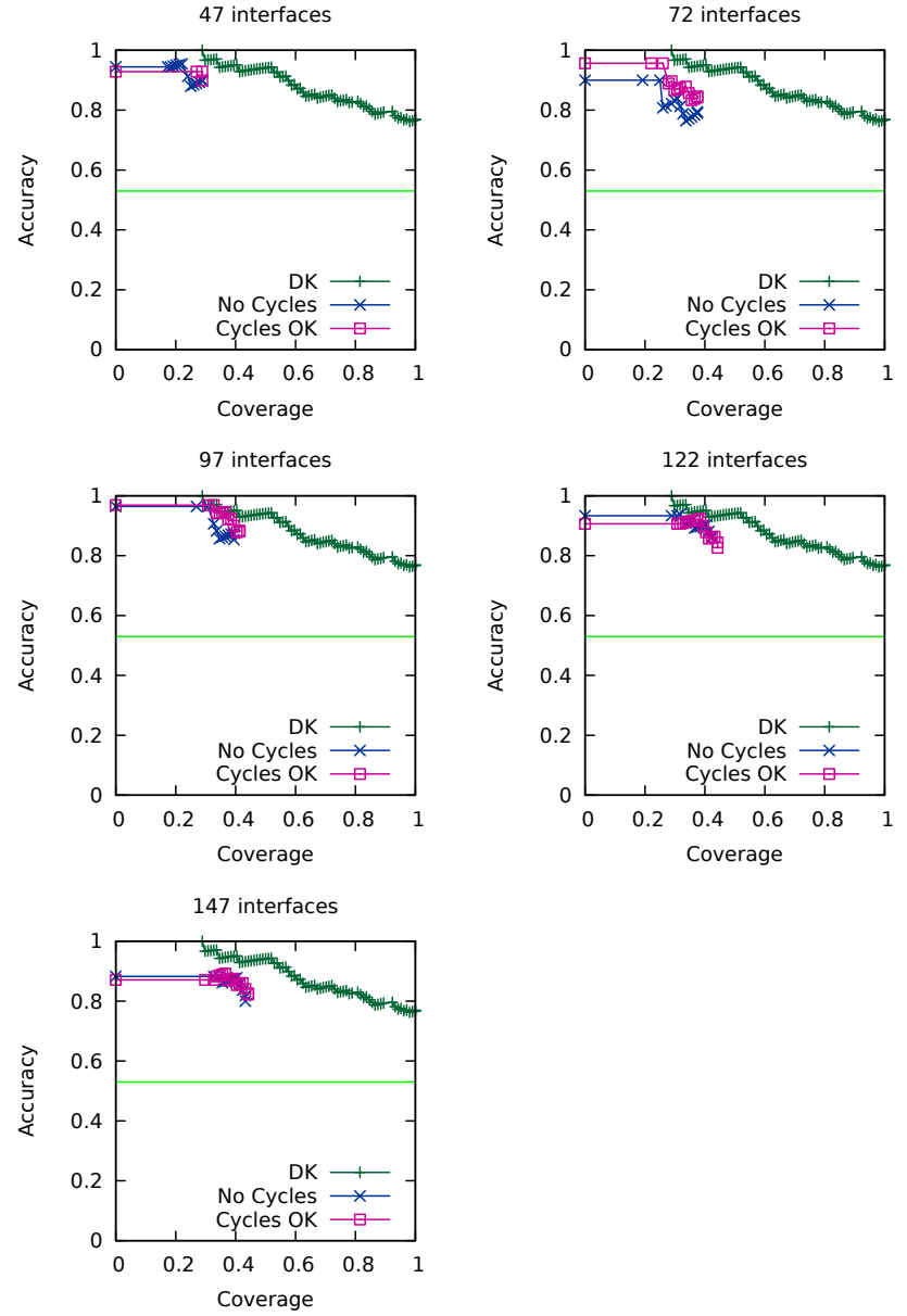
BMV Sign Prediction: Allowing or disallowing cycles ( \alpha=0.9 , using literature interactions)
