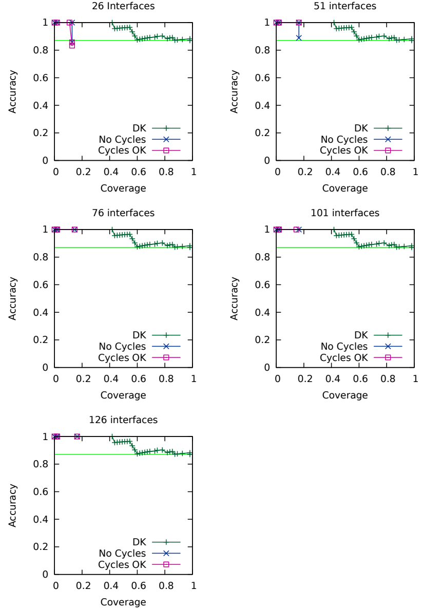
FHV Sign Prediction: Allowing or disallowing cycles ( \alpha=0.9 )
