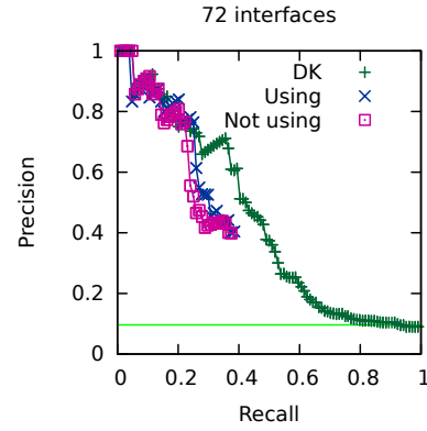
BMV Hit Prediction: Using literature interactions ( \alpha=0.9 , cycles disallowed)
