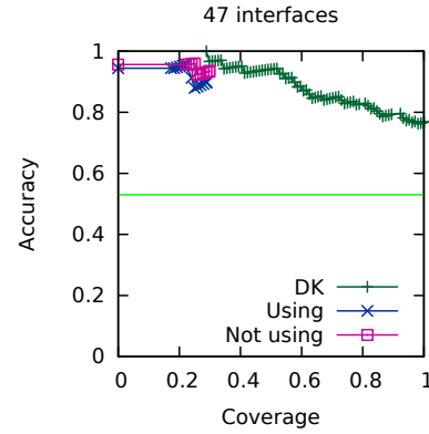
BMV Sign Prediction: Using literature interactions ( \alpha=0.9 , cycles disallowed)
