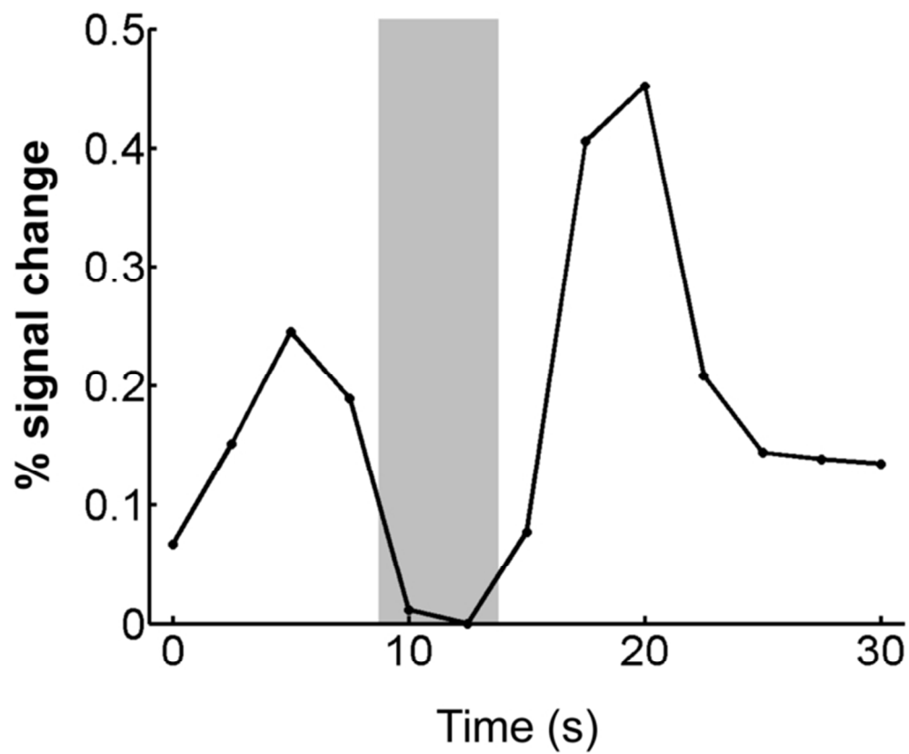
Figure S1. Responses in the visual cortex. Average estimated hemodynamic response (pooled over four conditions) from visual cortex ( x = 38 , y = -50 , z = -17 ) illustrating that activity at 10 and 12.5 sec post cue onset had minimal contribution from the transient cue phase. 62x52mm (300 x 300 DPI)
