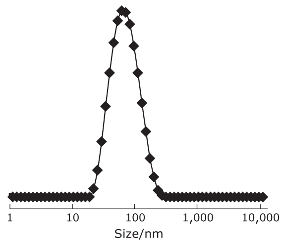
Supplemental Fig. 2. Size distribution of the RNP o analyzed by dynamic light scattering (DLS) (Malvern Instrument Ltd., UK) in aqueous media at 25°C. The RNP o thus obtained showed a unimodal distribution in the histogram analysis (41 nm, polydispersity index = 0.18).
