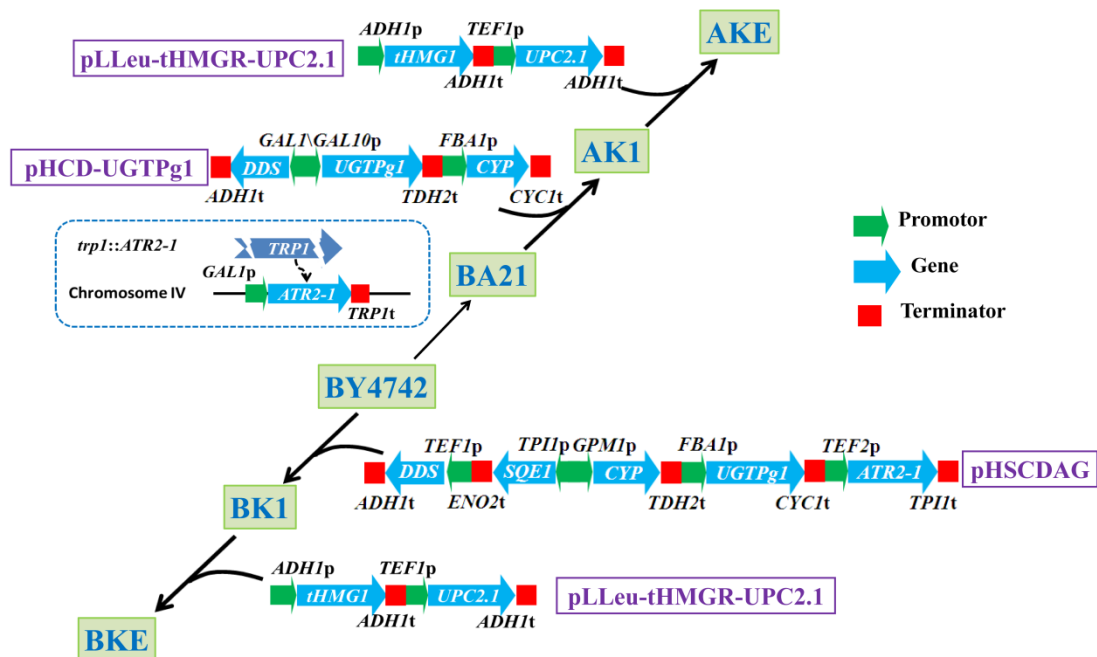
Supplementary Information, Figure S3. The construction of plasmids (A) and the recombinant yeast strains to yield CK (B) in this study.
