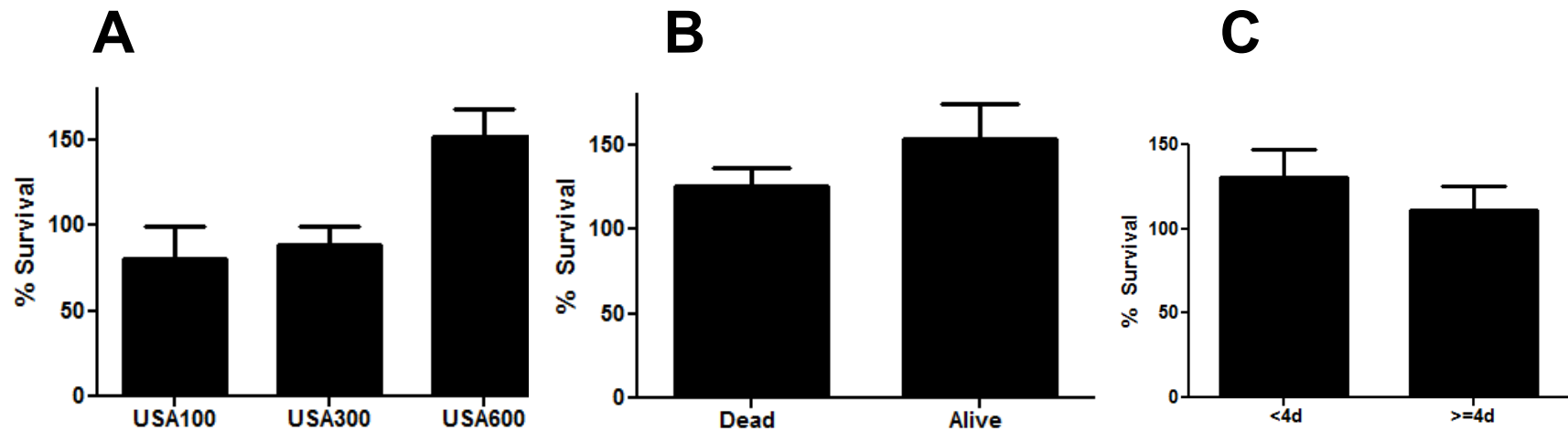
Supplemental Figure. Panel A: LL-37 (16 \mu M) killing assays of MRSA bloodstream isolates at 90 minutes, stratified by USA 600 versus USA 100 and USA 300 ( p=0.021 USA 600 vs USA100; p=0.017 USA 600 vs USA 300, Mann-Whitney U). Panel B: LL-37 survival of USA600 isolates from patients who died ( n=22 ) versus those who survived ( n=23 ). p=0.41 , Mann-Whitney U. Panel C: LL-37 survival of USA600 isolates from patients with bacteremia < 4 days ( n=14 ) versus \geq 4 days ( n=8 ). p=0.68 , Mann-Whitney U.
