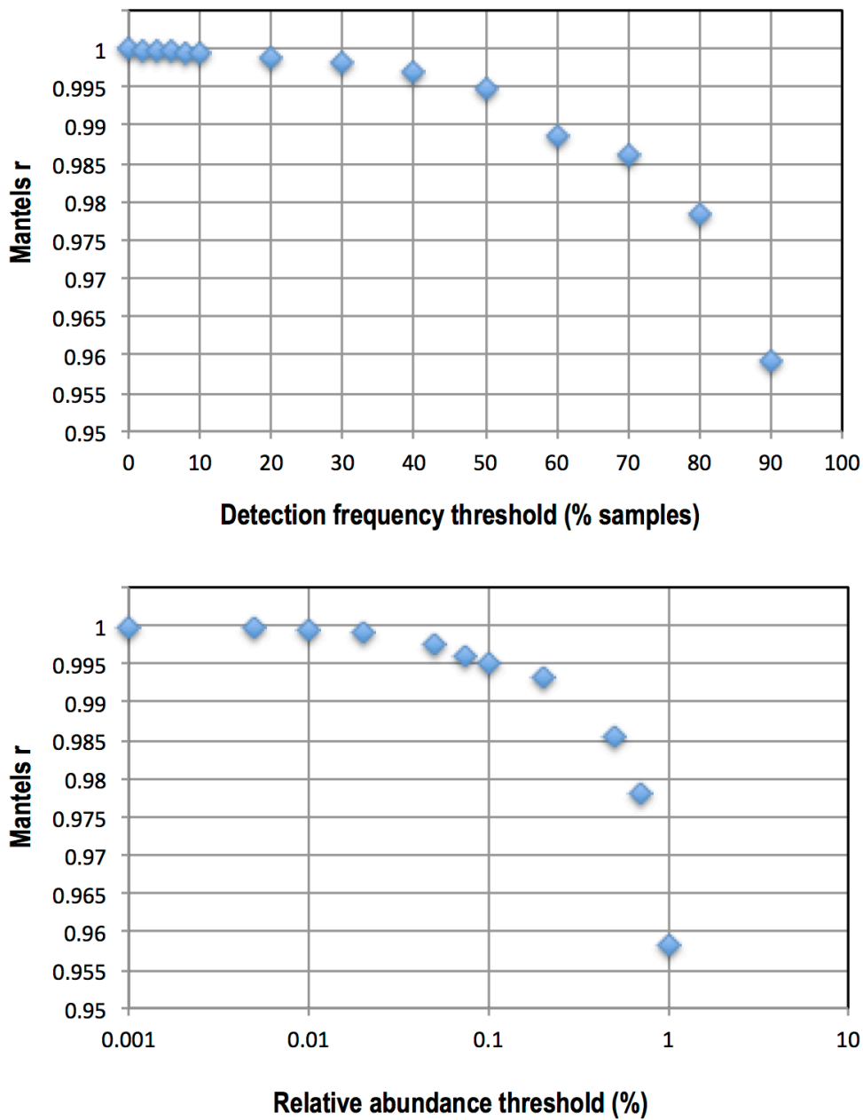
Supplementary Figure S3. Effect of OTU filtering based on detection frequency (top panel) and relative abundance threshold (bottom panel) on Mantels r . The lower the Mantel r , the lower the correlation between the full dataset with all OTUs and the dataset with subset of OTUs based on detection frequency or relative abundance threshold.
