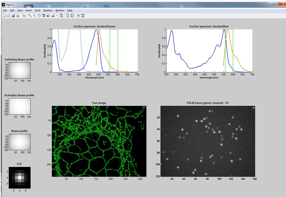
Figure S1 : View of our Matlab-based PALM simulation software. The microtubule pattern used to generate the data sets is shown in green. Spectroscopy data characterizing the used PTFP are shown on the top, here for Dendra2 in its green state (left) and in its red state (right). The PSF and the beam profiles of the various lasers used in the simulated experiment are shown on the left column.
