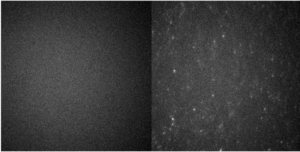
Figure S2 : Representative frames from a PALM dataset of a “blank” PVA sample devoid of Dendra2 molecules (left) and a PVA sample containing Dendra2 (right). No blinking molecule can be noticed on the left image. Images are acquired under the same experimental conditions.
