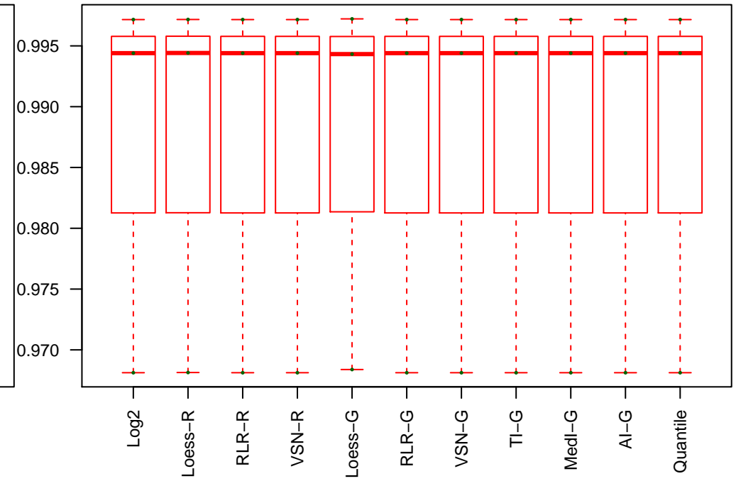
Spearman correlation – Intragroup
