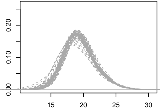
TI-G
