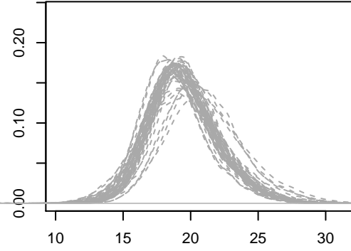
RLR-R
