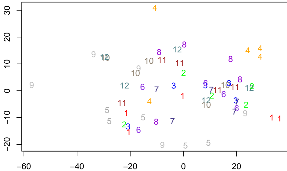
Log2-MDS plot
