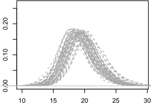
Log2
