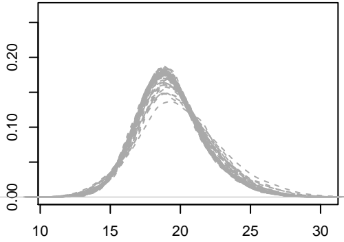
Loess-G
