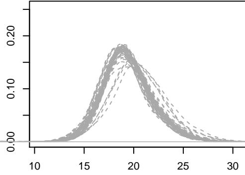
Loess-R
