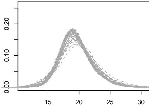
RLR-G
