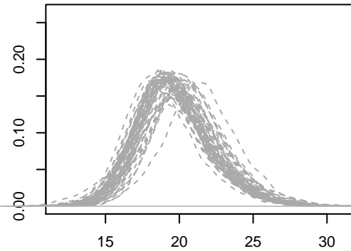
NF-G
