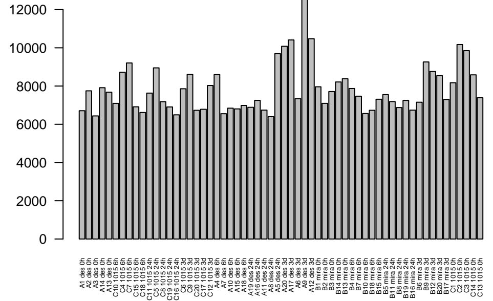
Total missing
