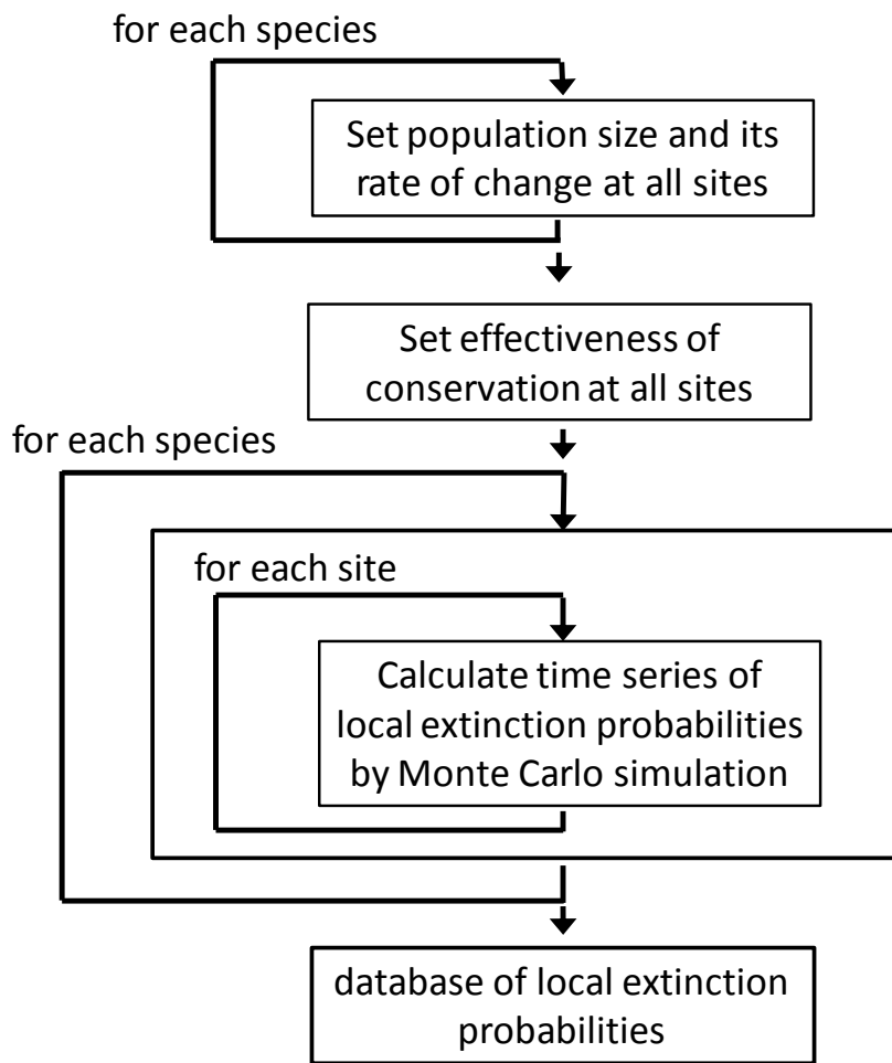
Figure S1 Preparation of database of probabilities of local extinction in SPERS.
