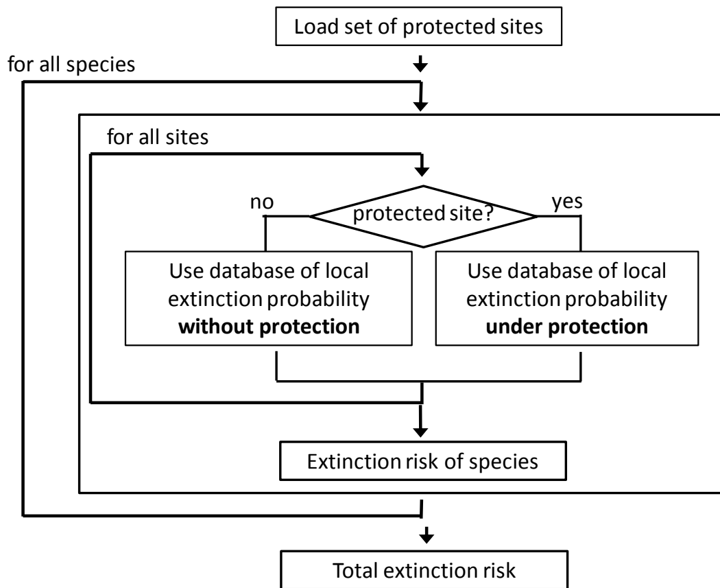
Figure S2 Estimation of extinction risks under the given set of protected sites in SPERS.
