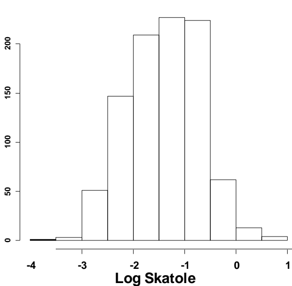
Supplementary Figure 1 Histograms of skatole (left) and androstenone (right), untransformed (top) and log transformed data (bottom).
