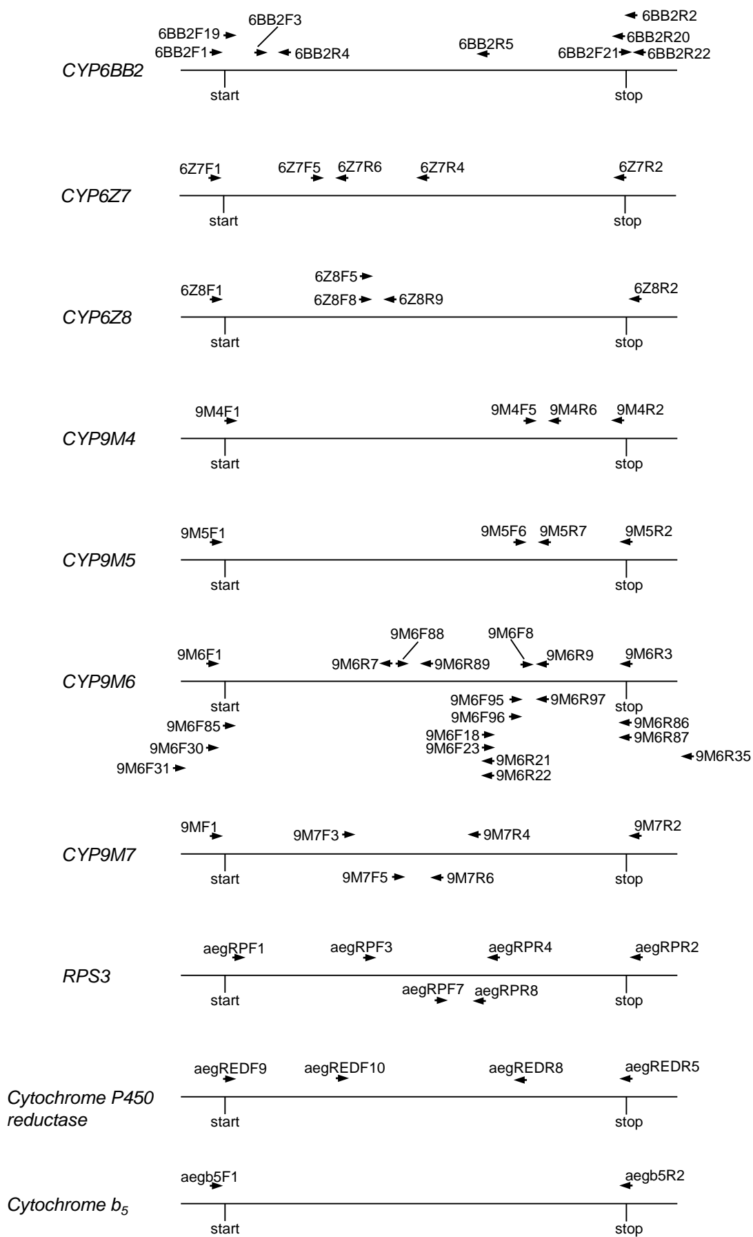
Figure S1 Diagram depicting primer positions
