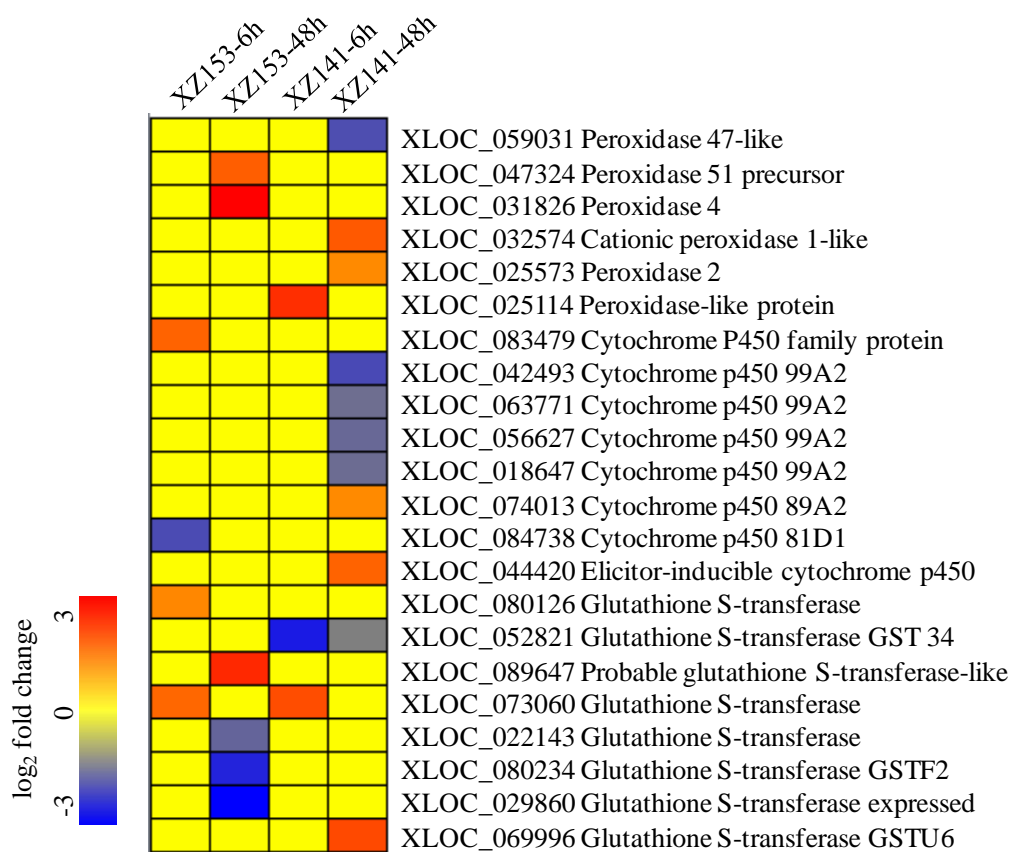
Figure S4. Heat Map analysis of DEGs involved in oxidative stress-related in XZ153 and XZ141. The sample and treatments are displayed above each column. Genes are displayed by different colors. Relative levels of expression are shown by a color gradient from low (blue) to high (red).
