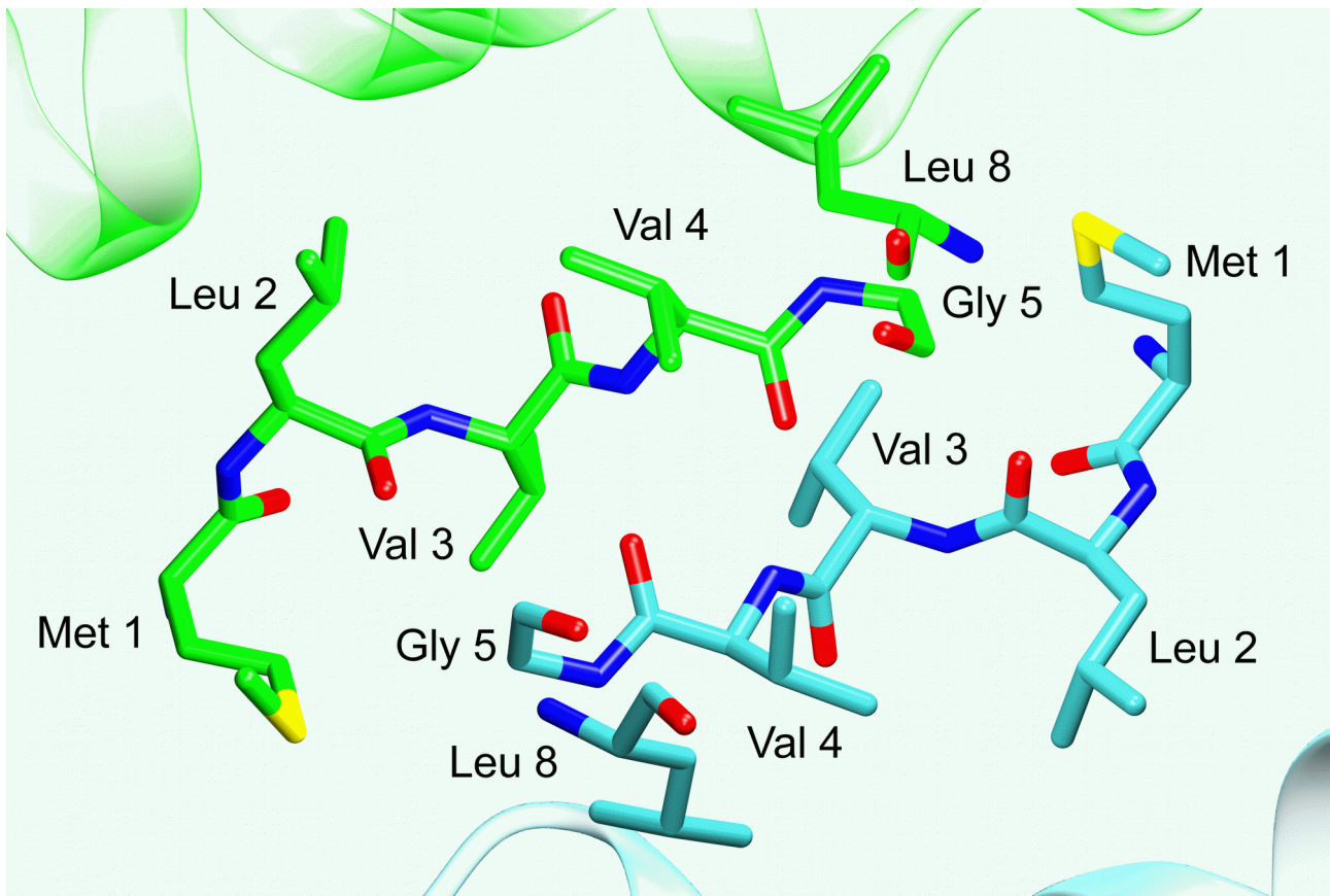
Fig. 1S. Two antiparallel arrays of N-terminal non-polar residues stabilizing the molecular crystal packing of the mTS-dUMP-Raltitrexed complex structure.
