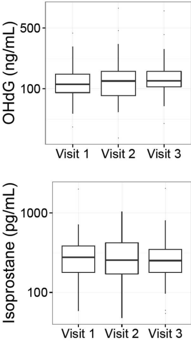
Figure S1. Boxplots comparing oxidative stress biomarker distributions by study visit.
