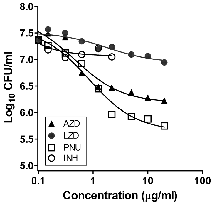
Supplementary FIG. 2. Bactericidal activity of three oxazolidinones against hypoxic non-replicating M. tuberculosis .
