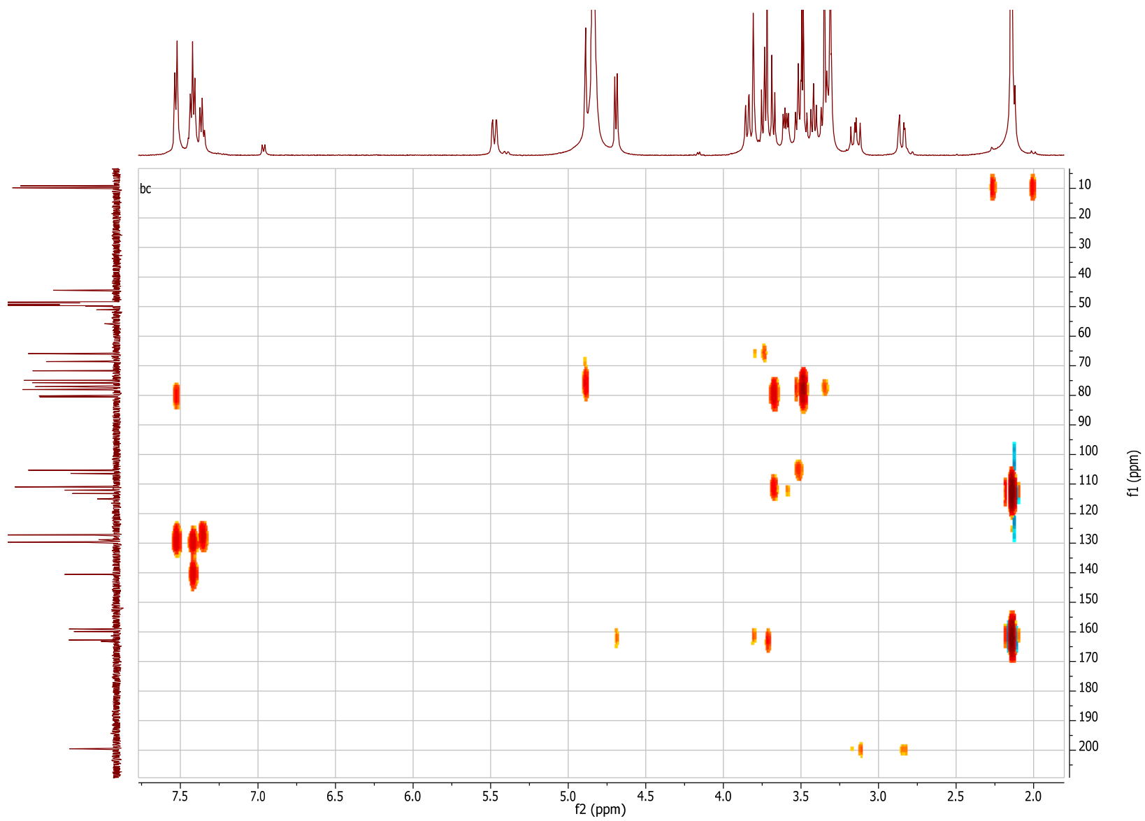
Fig. 6S. HMBC experiment of compound 1.
