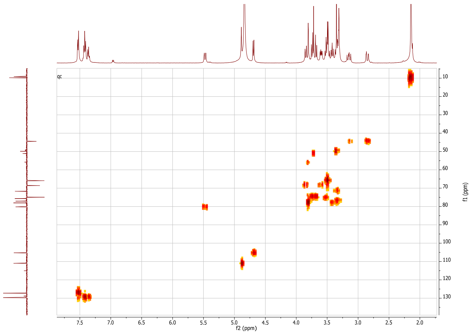
Fig. 5S. HSQC experiment of compound 1 .
