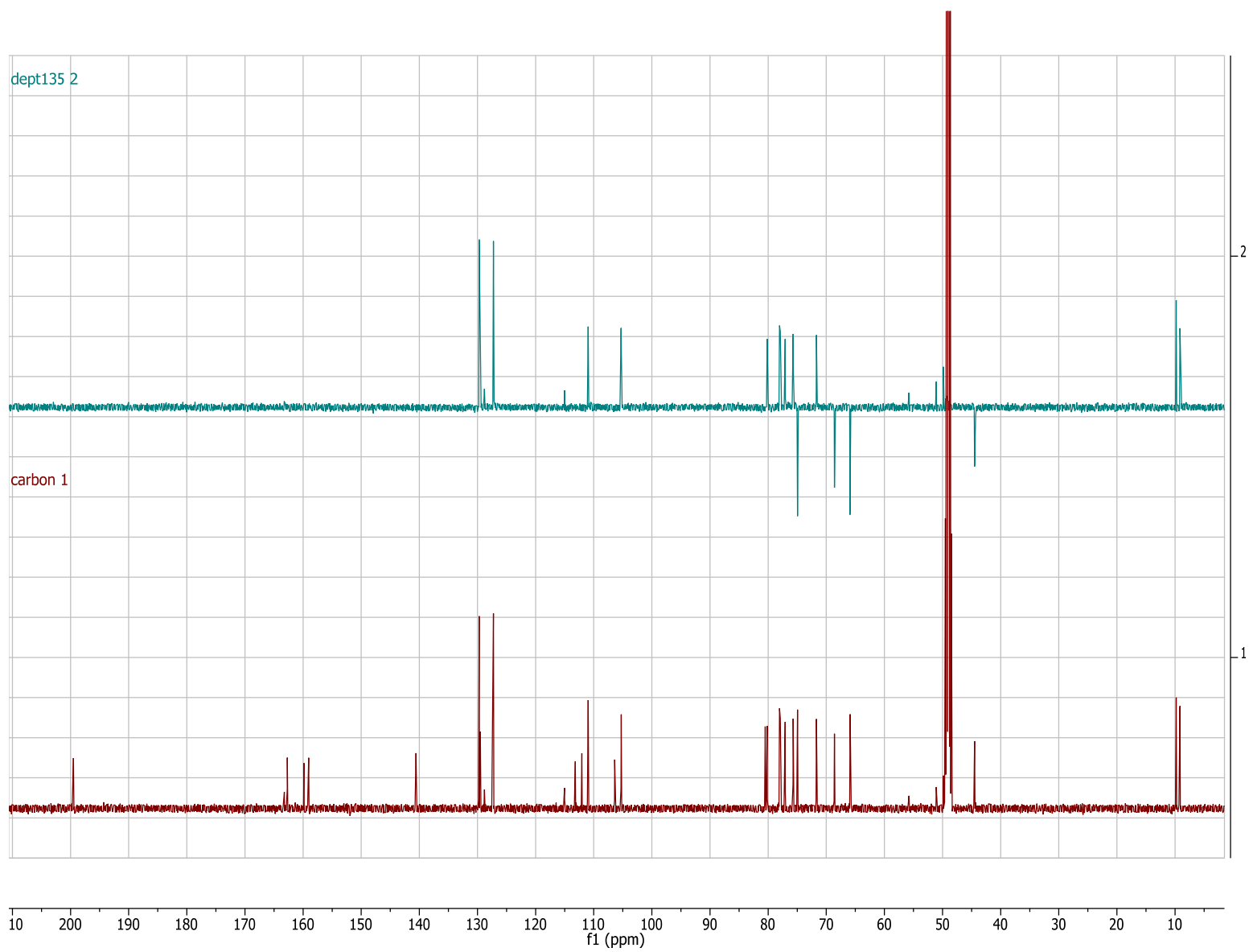
Figure 3S. 13 C NMR y DEPT experiments of compound 1.
