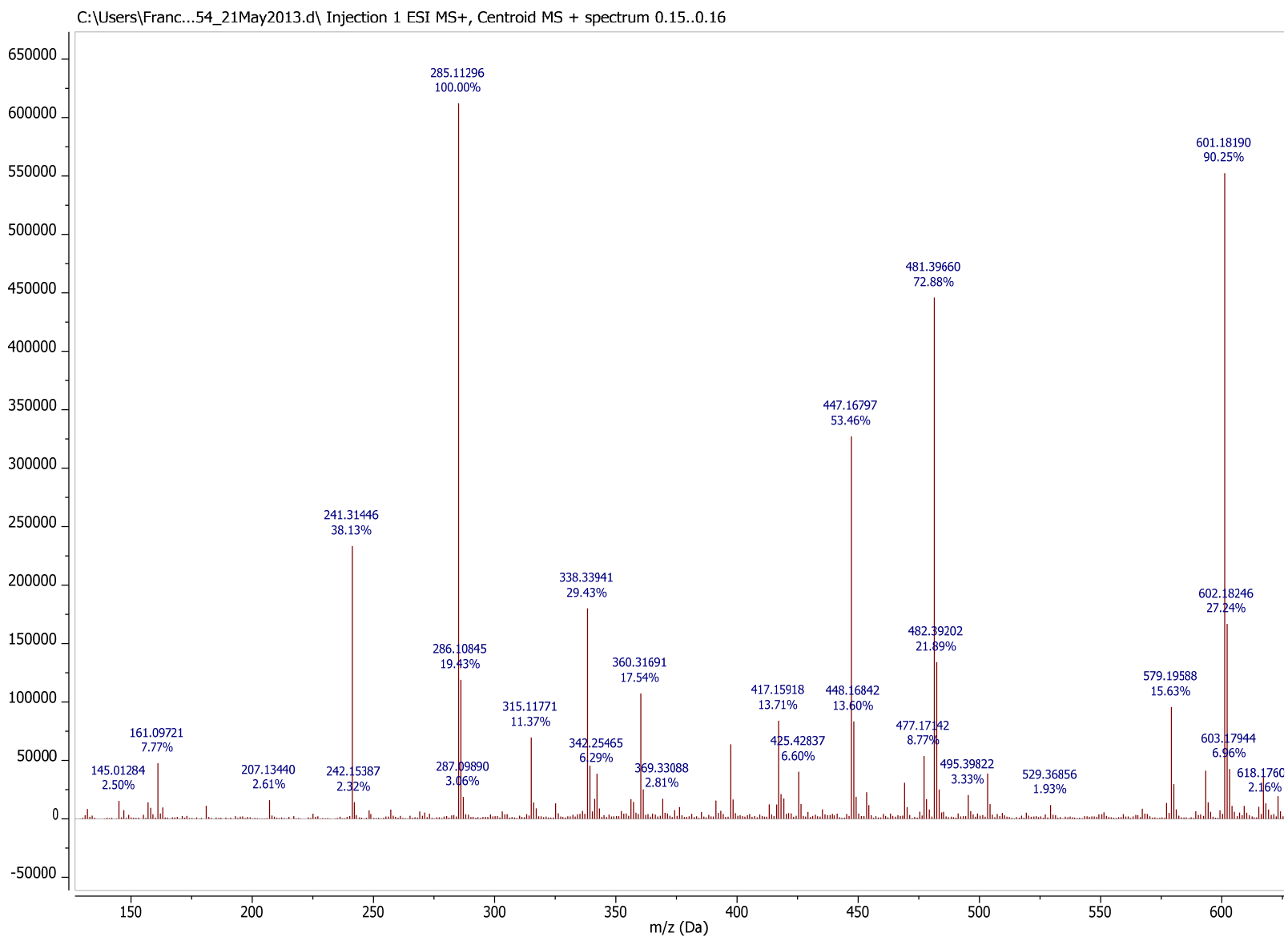
Fig. 7S. HR-ESIMS of compound 1 .
