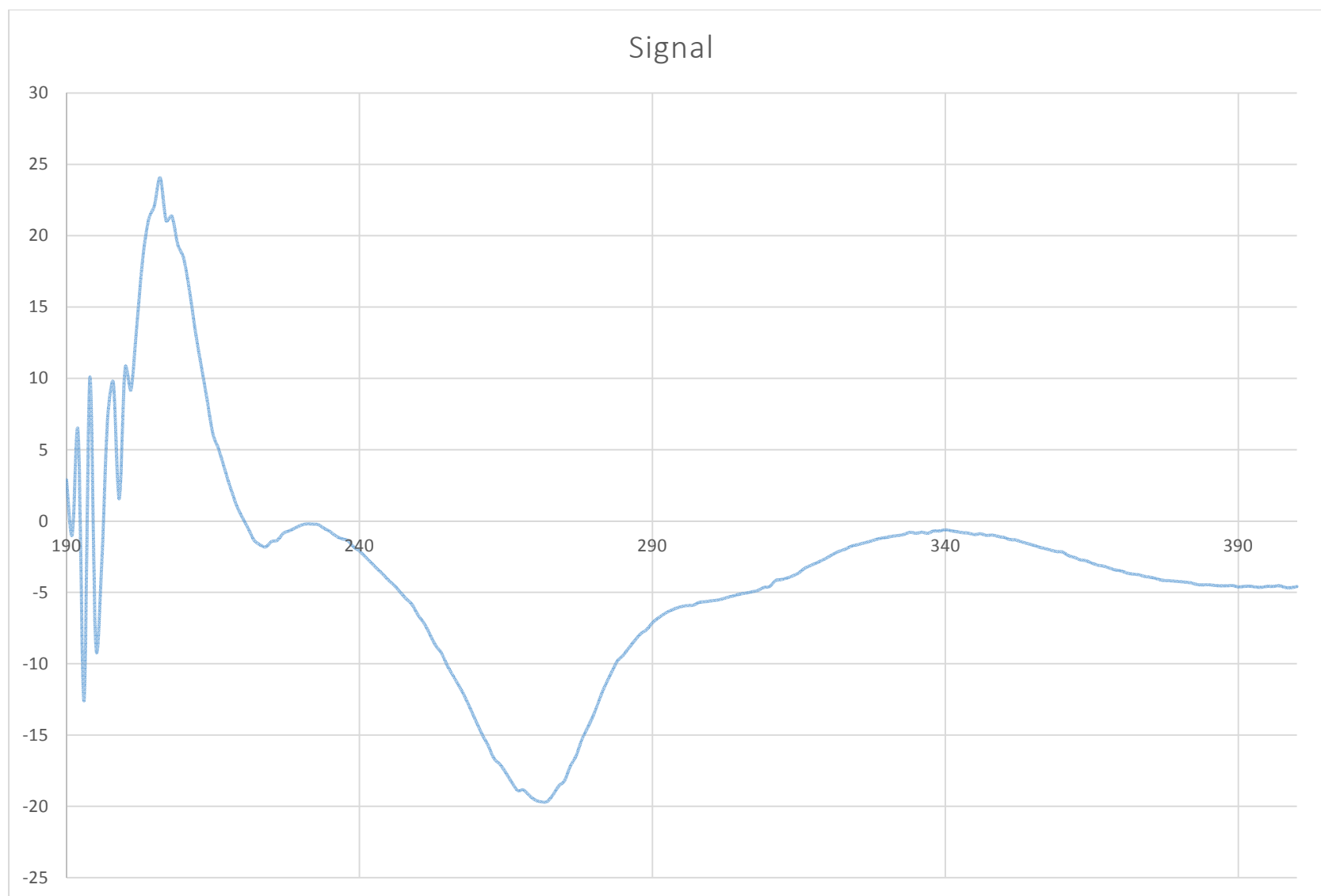
Fig. 8S CD Experiment of compound 1.
