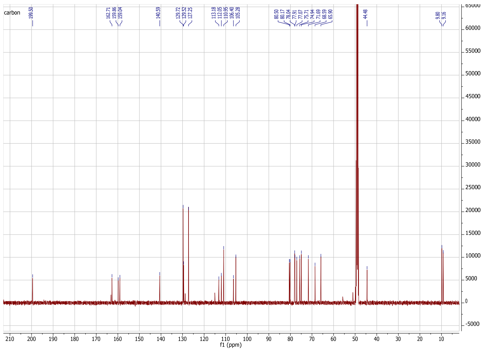
Fig. 2S ^{13}\text{C} NMR of compound 1 .
