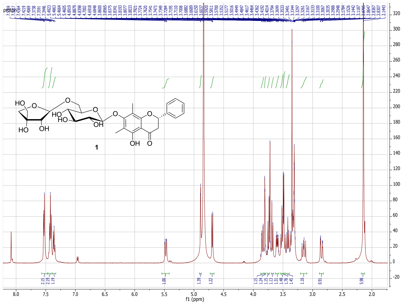
Fig. 1S ^1\text{H} NMR of compound 1.
