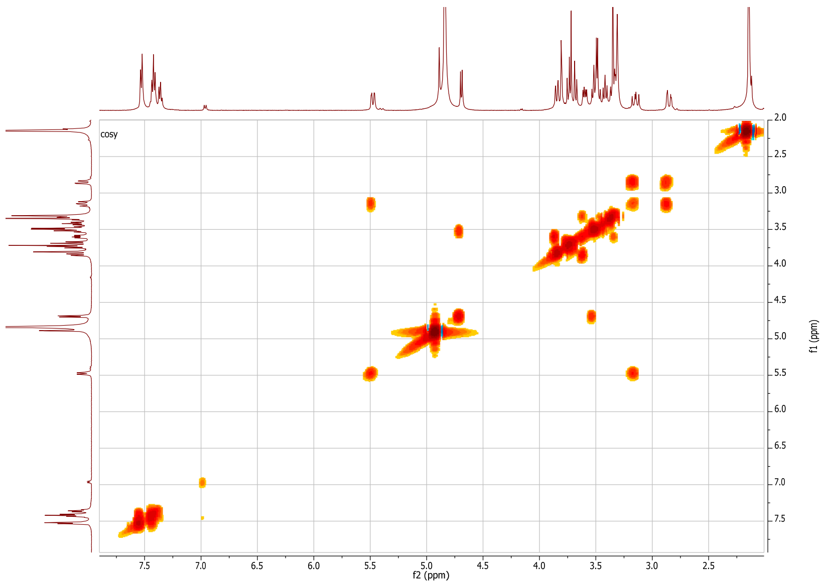
Fig. 4S COSY experiment of compound 1 .
