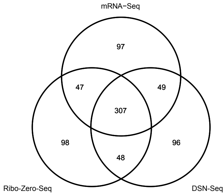
Figure S3. Comparison of the top 500 differentially expressed genes between Basal and Luminal tumors detected by mRNA-Seq, Ribo-Zero-Seq and DSN-Seq.
