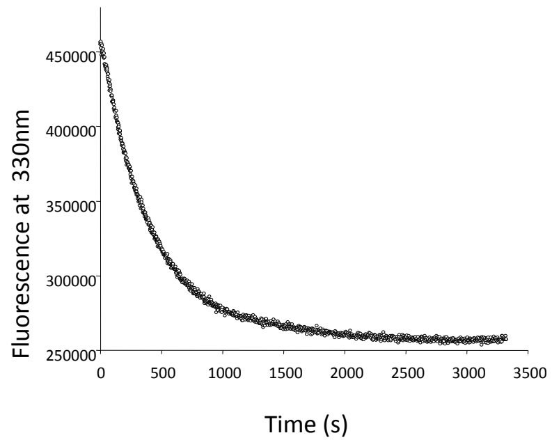
(a) Fluorescence of the tryptophan for the phosphatase domain of PHLPP2 was recorded as a function of time following treatment with 100 mM EDTA. The reduction of fluorescence reflects unfolding of the protein, exposing some tryptophans.
