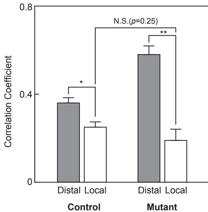
Figure S6, Place field similarity measurements in distal cue- and local cue-centric coordinate frames.
