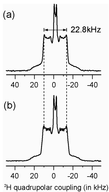
Figure S1. Static ^2\text{H} powder spectra of d_{54} -DMPC/DMPG membrane without (a) and with (b) penetratin at 310 K.
