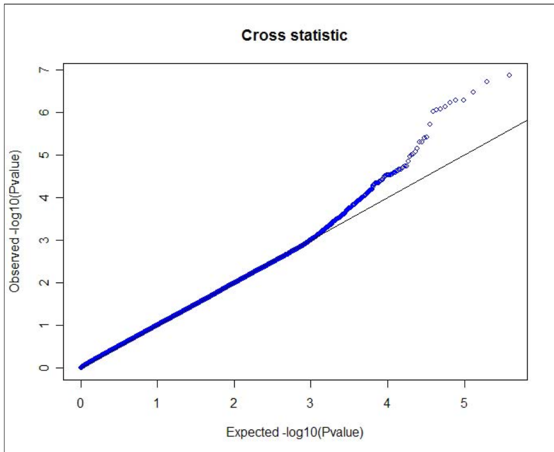
Supplemental Figure 3: Observed vs. expected -\log_{10}(\text{P-value}) s across the genome for the cross statistic.
