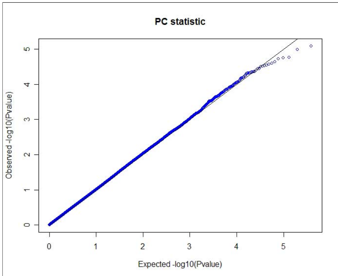
Supplemental Figure 2: Observed vs. expected -\log_{10}(\text{P-value}) s across the genome for the pc statistic.
