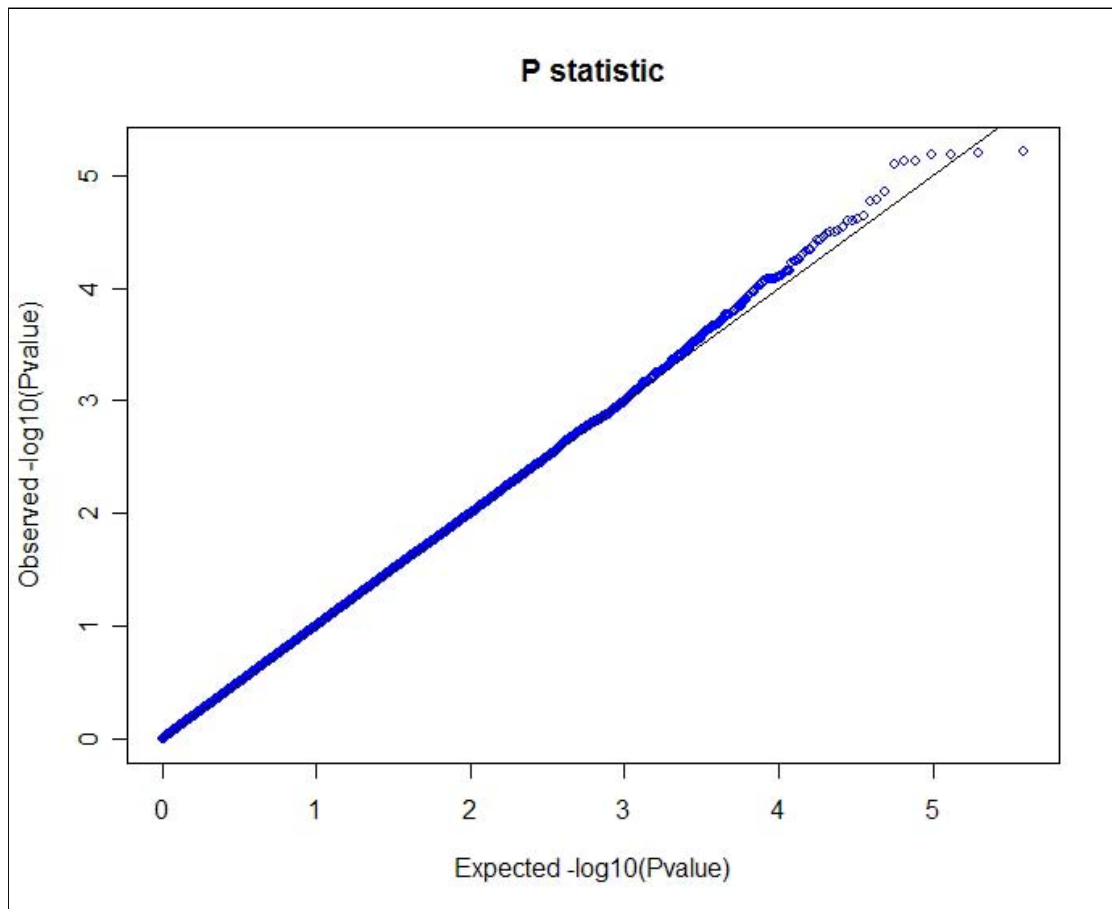
Supplemental Figure 1: Observed vs. expected -\log_{10}(\text{P-value}) s across the genome for the p statistic.
