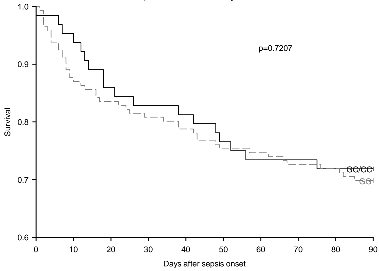
Kaplan-Meier survival analysis
