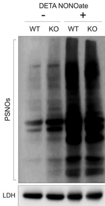
SUPPLEMENTARY FIG. S1. Reliability of the biotin-switch assay. Evaluation of protein S -nitrosothiols (PSNOs) amount in total homogenates of tibialis anterior of 2-month-old GSNOR-KO (KO) and wild-type (WT) mice, treated with (+) or without (-) 2 mM DETA NONOate for 30 min at room temperature. On incubation, lysates were subjected to biotin-switch assay and revealed by incubation with HRP-conjugated streptavidin. LDH was selected as a loading control.
