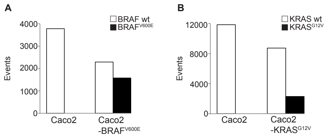
Figure S1: Successful transfection of pMCEF-BRAF V600E or pcDNA3-KRAS G12V into Caco2 colon cancer cell line. BRAF V600E (A) or KRAS G12V (B) was detected by digital droplet PCR, using the Bio-RadQX200 ddPCR platform.
