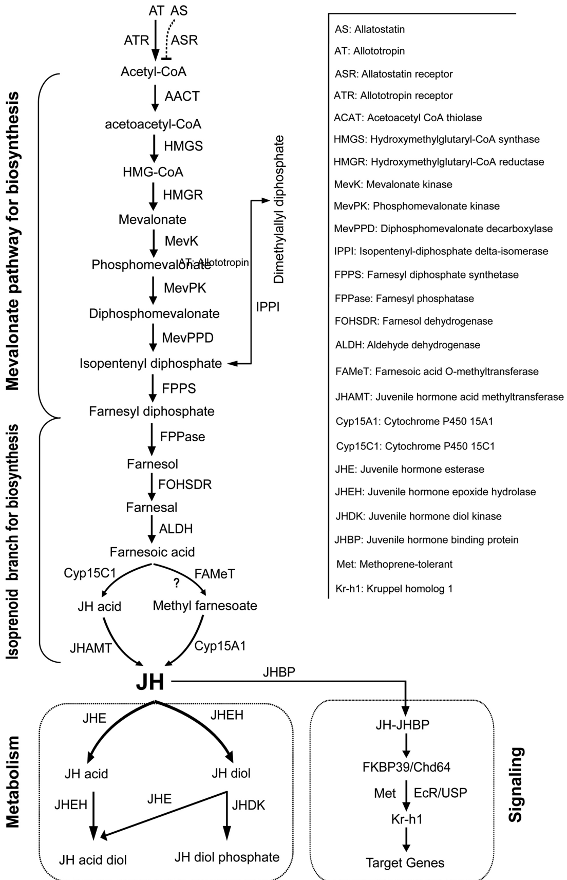
Figure S1 - Summary of insect JH-related pathways. Taken into account previous reports, we summarized the main steps in the pathways related to the biosynthesis, metabolism, and signaling of JH in insects.
