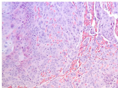
Tongue (200x)
