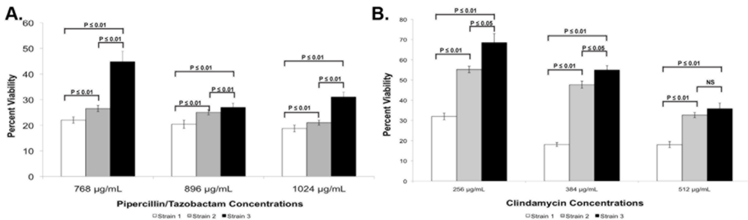
Fig S1A. Compared to strain 1, strains 2 and 3 are significantly more resistant to piperacillin/tazobactam, though it should be noted that these very high concentrations are not clinically relevant. B. Compared to strain 1, strains 2 and 3 are significantly more resistant to clindamycin.
