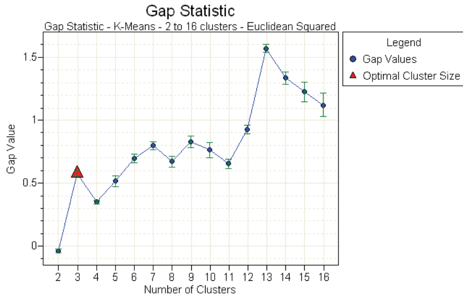
Figure S2. Gap statistic analysis of UV-differentially expressed genes in Tempranillo berry skin. The Gap score for each cluster number (between 2 and 16) using k-means clustering and Euclidean squared metrics is shown. The resulting optimum number of clusters is highlighted by a red triangle.
